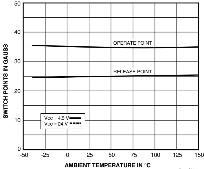
SWITCH POINTS
