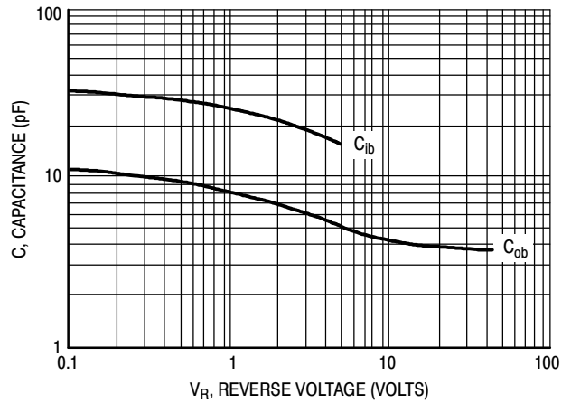
Figure 5. Capacitances
