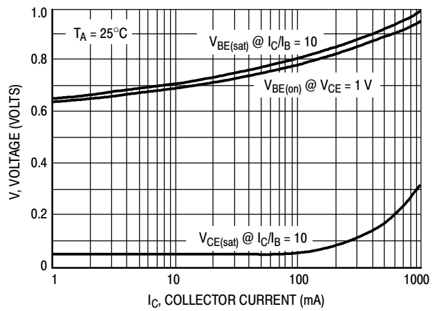
Figure 3. "On" Voltages
