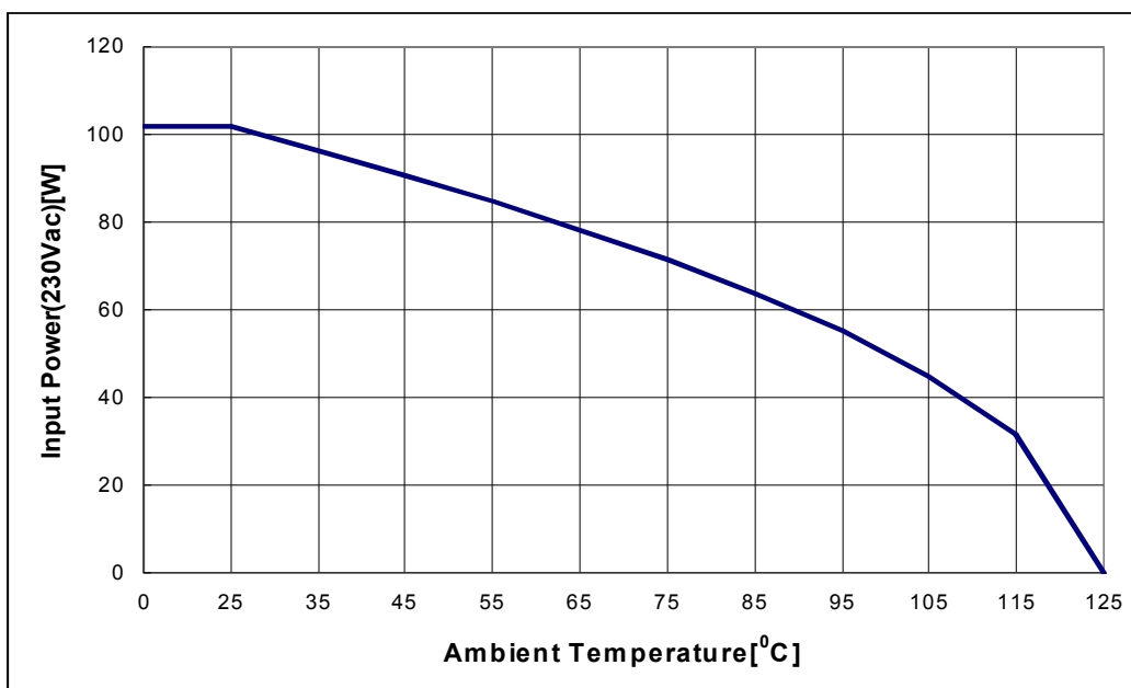
Figure 13 Input Power curve V_{in}=230\text{Vac}; P_{in}=f(T_a)
