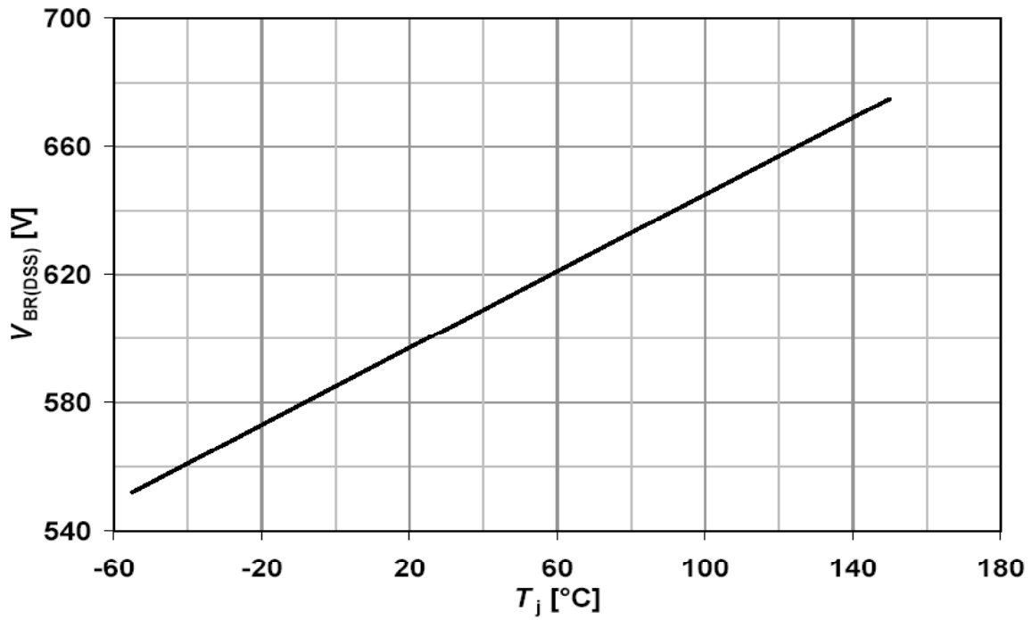
Figure 11 Drain-source breakdown voltage; V_{BR(DSS)}=f(T_j)
