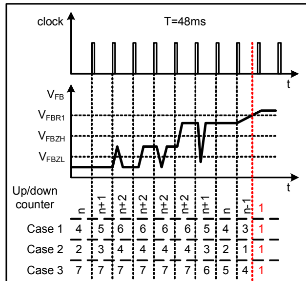
Figure 5 Up/down counter operation
