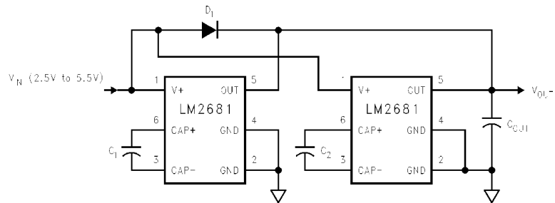
FIGURE 3. Lowering Output Resistance by Paralleling Devices
