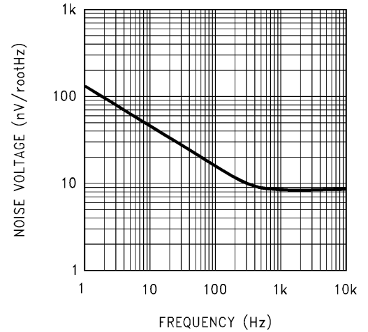
Noise Voltage vs. Frequency
