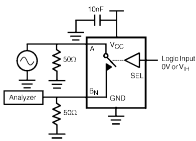
FIGURE 5. Off Isolation
