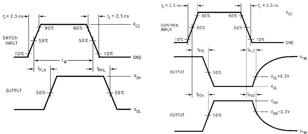
FIGURE 2. AC Waveforms
