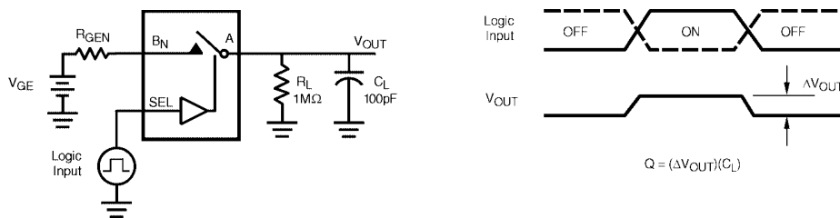
FIGURE 4. Charge Injection Test
