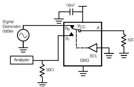
FIGURE 6. Crosstalk
