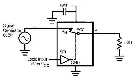
FIGURE 9. Bandwidth
