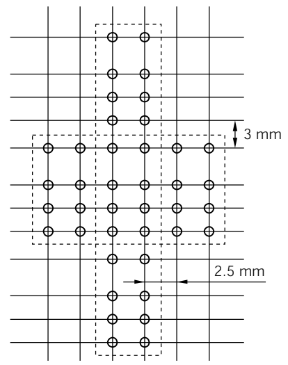
Mounting space
