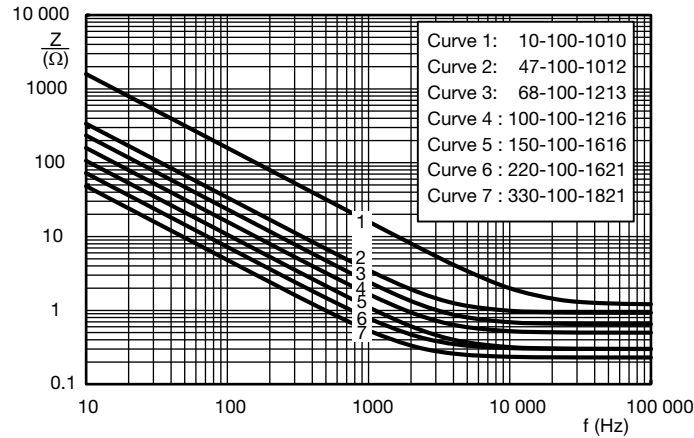
Fig. 10 - Typical impedance as a function of frequency
