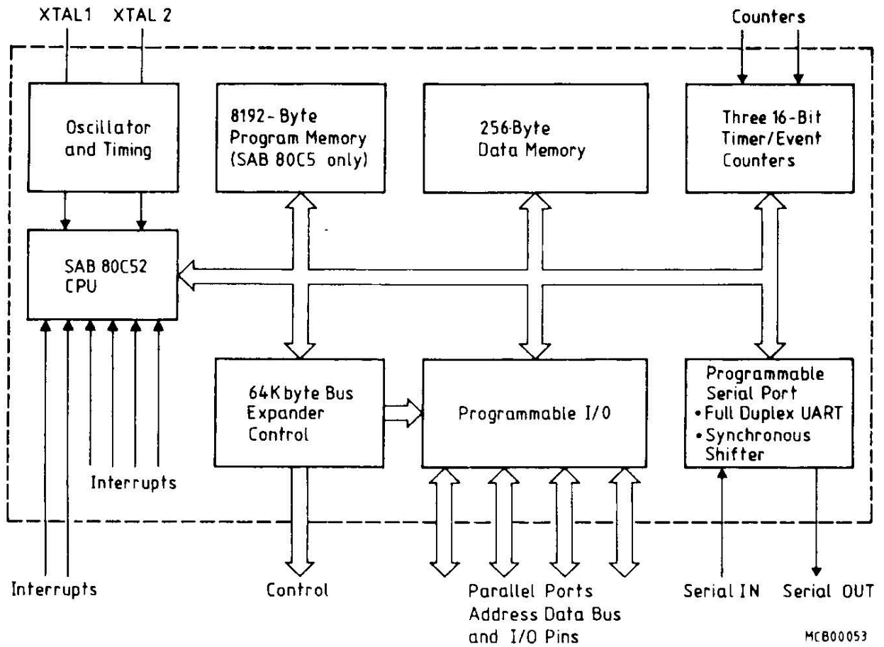
Figure 1 Block Diagram
