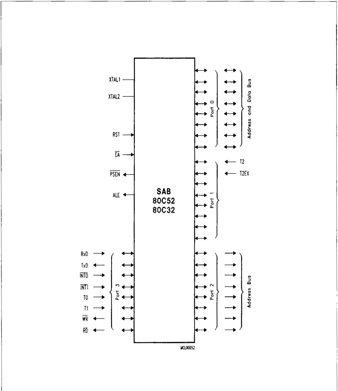
Logic Symbol
