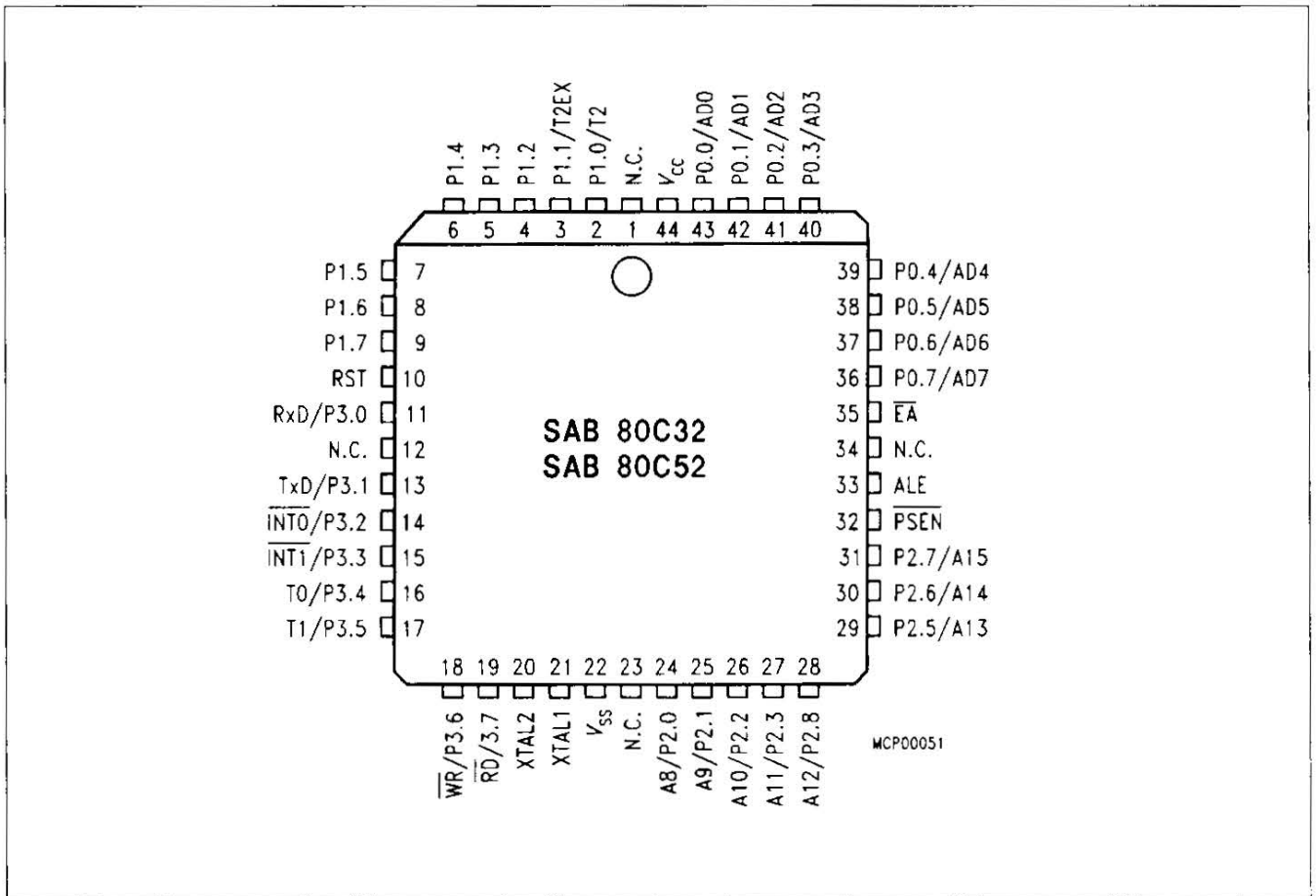
Pin Configuration (P-LCC-44)
