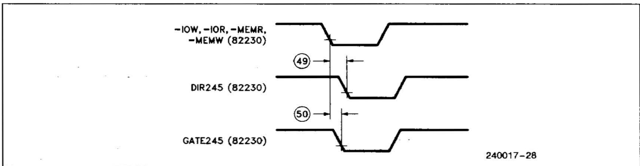
Figure 14. 82230 DIR245, GATE245 Timing
