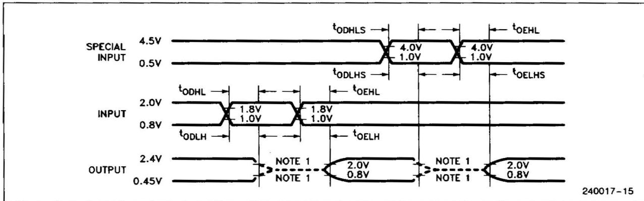
Figure 1C. Output Enable/Disable Time Measurement
