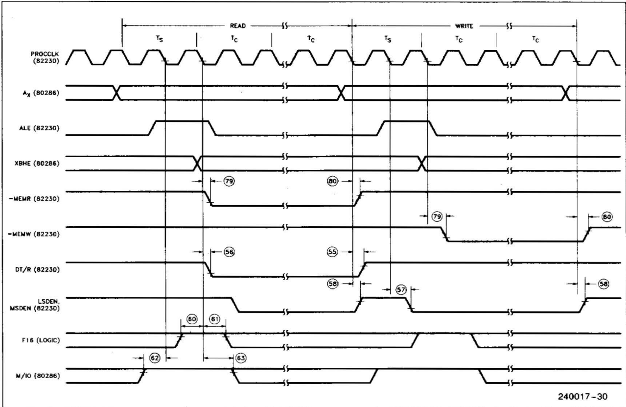
Figure 16. Memory Read/Write Cycles
