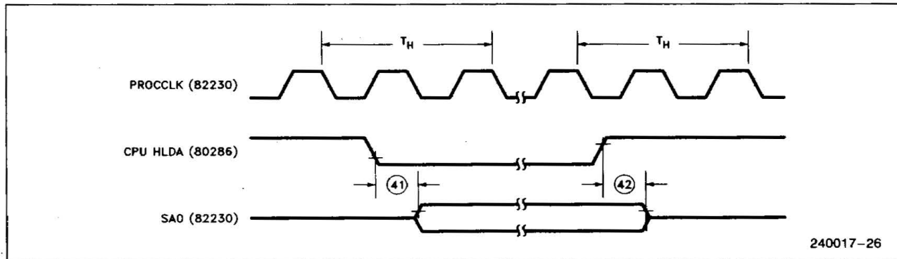
Figure 12. 82230 SA0 Timing
