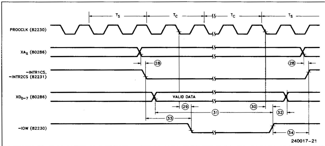
Figure 7. 82230 8254 Bus Write Timing
