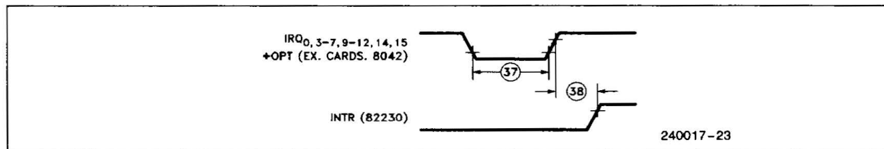
Figure 9. Interrupt Request Timing
