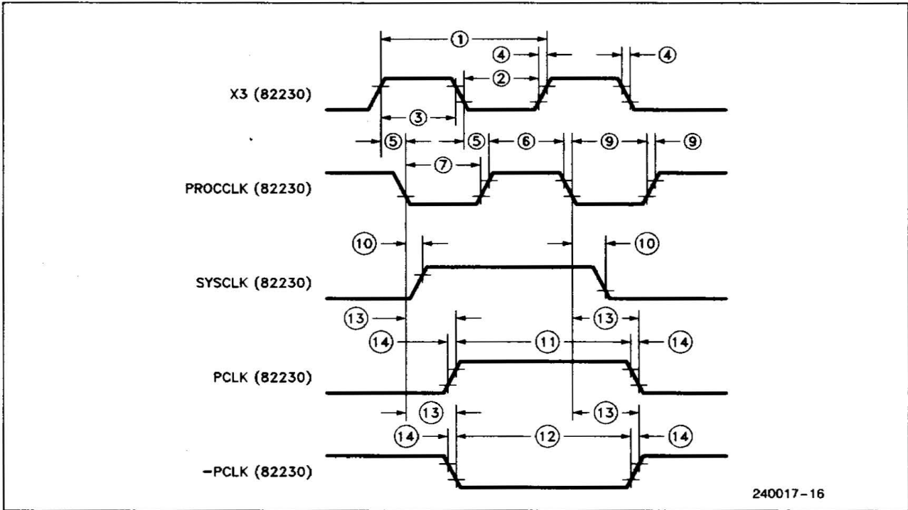
Figure 2. 82230 Clock Timing
