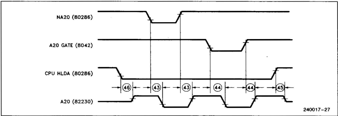
Figure 13. 82230 A20 Timing
