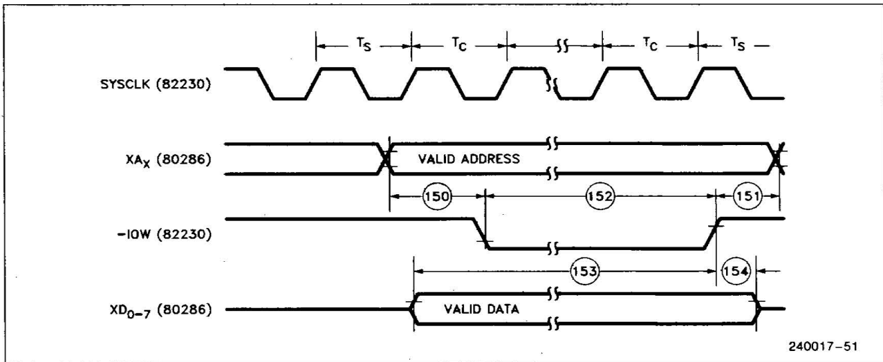
Figure 37. 82231 CPU Write Timing
