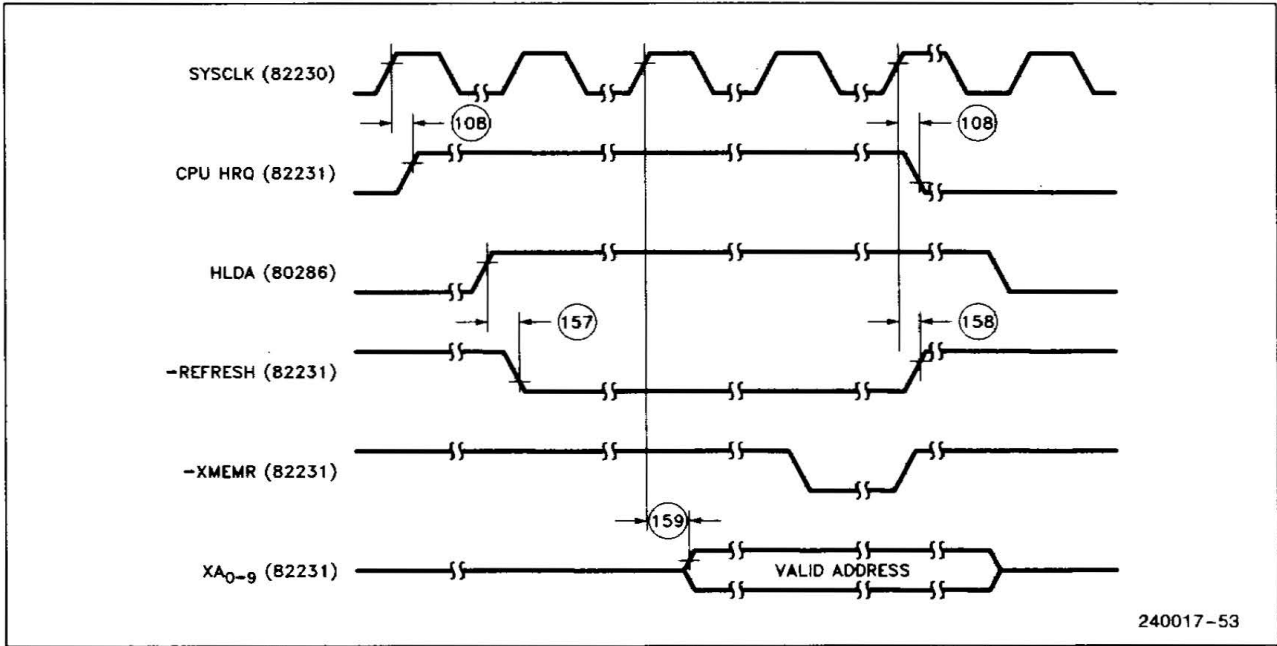
Figure 39. 82231 REFRESH Timing
