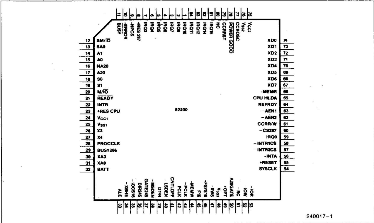
Pin Diagram 82230
