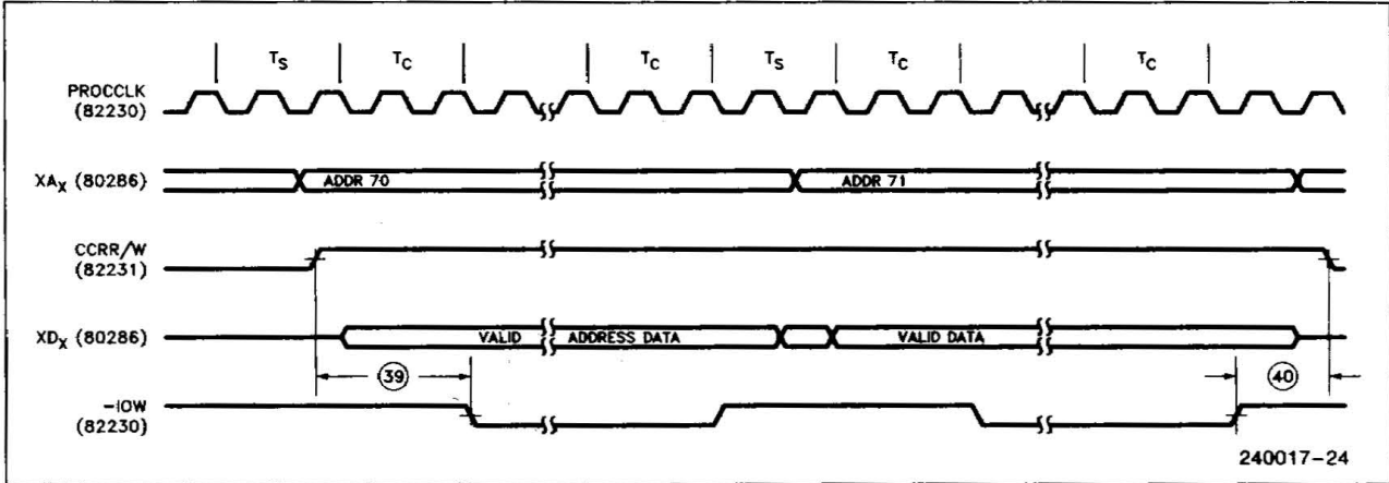
Figure 10. 82230 6818 Write Cycle
