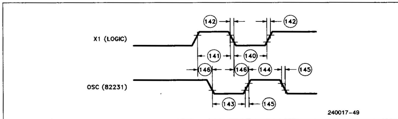
Figure 35. X1 and OSC Timing
