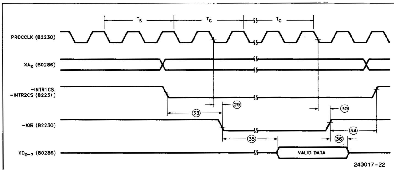
Figure 8. 82230 8254 Bus Read Timing
