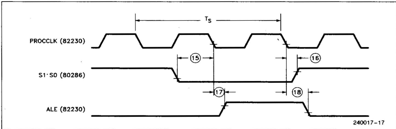
Figure 3. 82230 Status and ALE Timing
