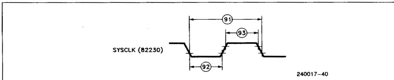
Figure 26. 82231 SYSCLK Timing
