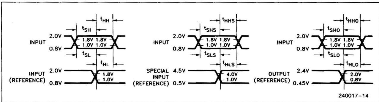
Figure 1B. Setup/Hold Time Measurements
