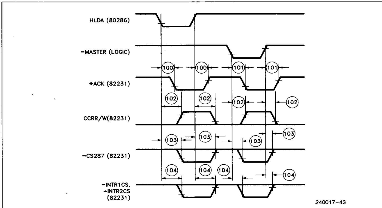
Figure 29. 82231 HLDA & - MASTER Timing
