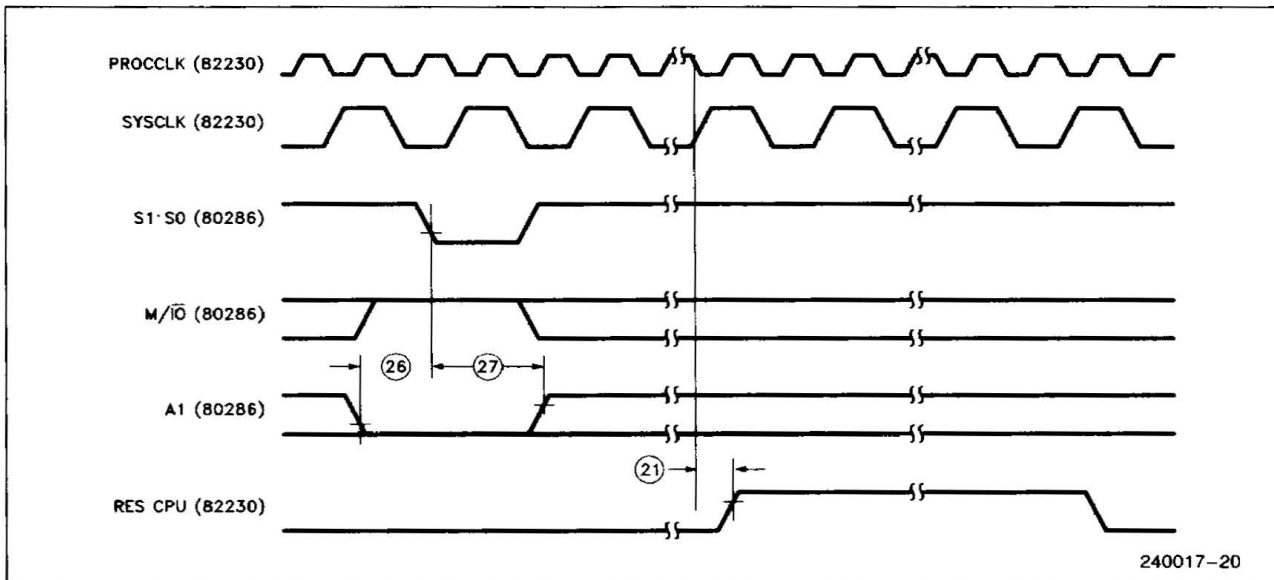
Figure 6. 82230 Processor Shutdown Initiated Reset
