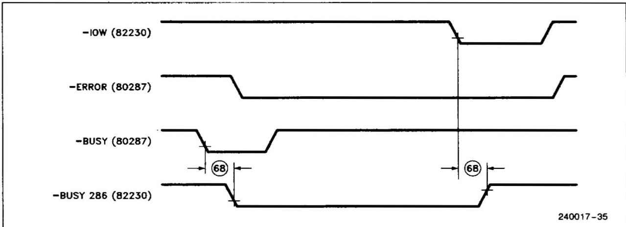
Figure 21. -BUSY286 Timing
