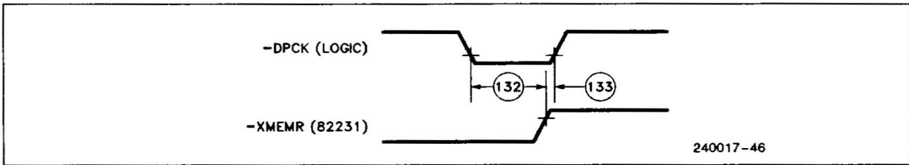
Figure 32. 82231 DPCK Timing
