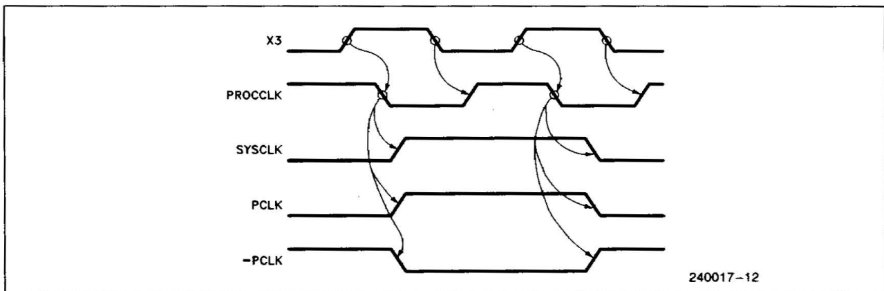
Figure 2. 82230 Clock Timing
