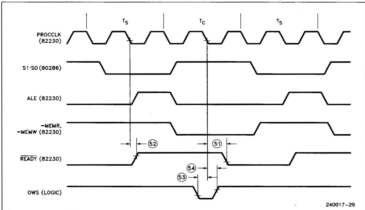
Figure 15. 82230 Zero Wait State Timing
