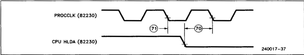
Figure 23. 82230 CPU HLDA Timing
