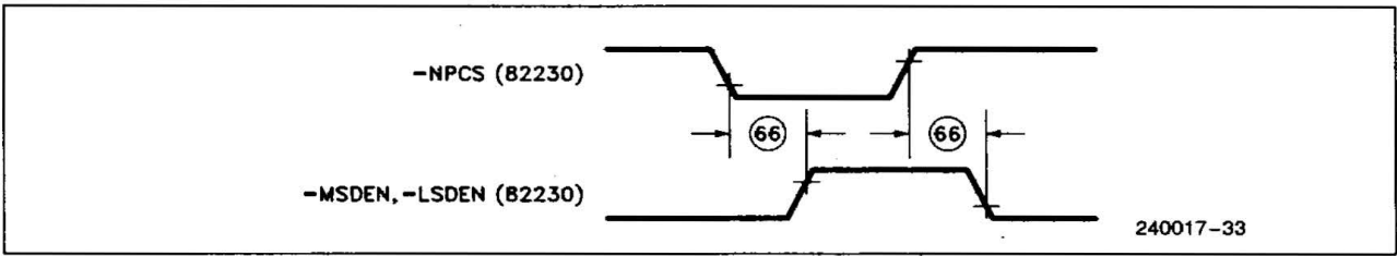
Figure 19. 82230 MSDEN, LSDEN Timing
