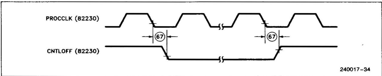
Figure 20. CNTLOFF Timing
