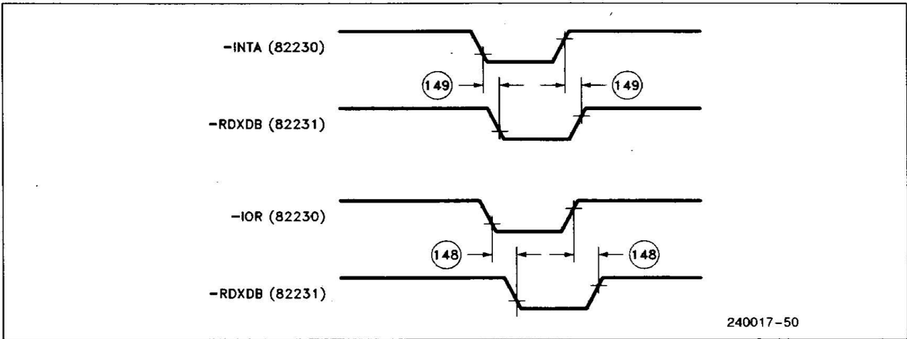
Figure 36. 82231 RDXDB Timing
