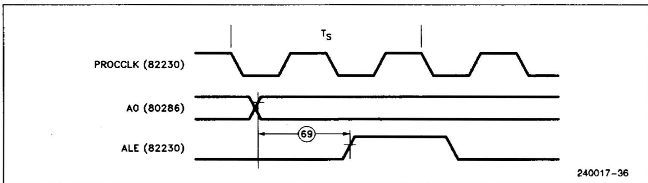
Figure 22. 82230 A0 Timing
