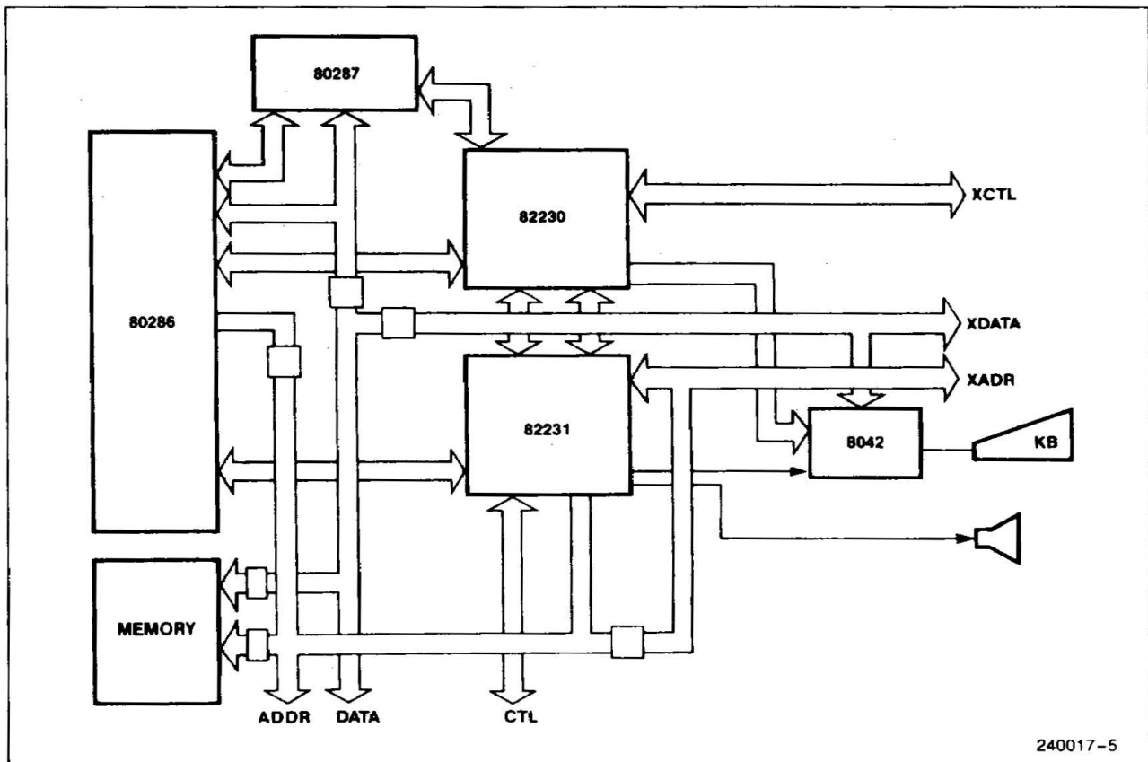
Figure 1. Block Diagram of 82230 and 82231 for PC/AT
