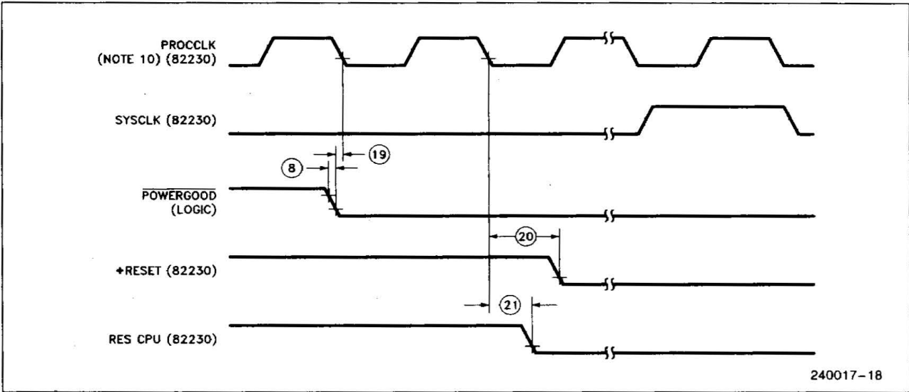
Figure 4. 82230 Power on Initiated Reset
