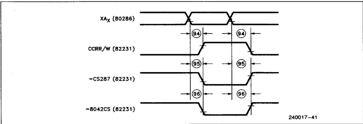
Figure 27. 82231 CCRR/W and CS287 Timing
