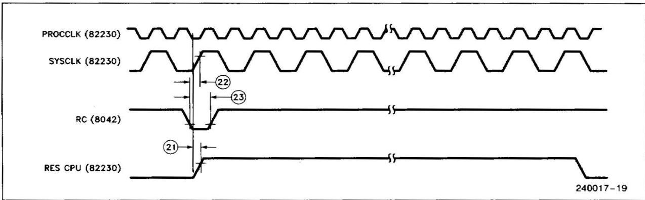
Figure 5. 82230 Keyboard Initiated Reset
