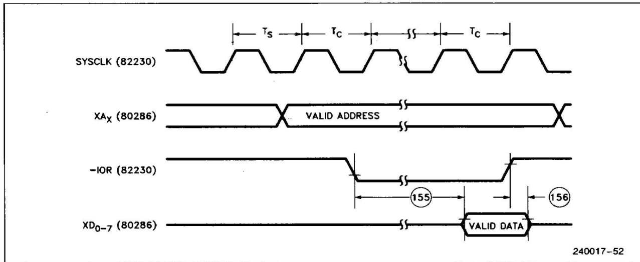
Figure 38. 82231 CPU Read Timing
