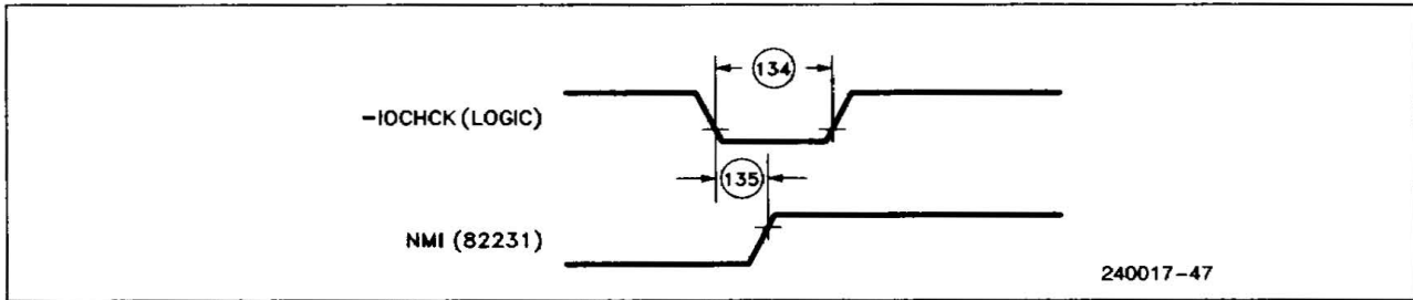
Figure 33. 82231 IOCHCK and NMI Timing
