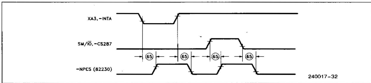
Figure 18. 82230 NPCS Timing
