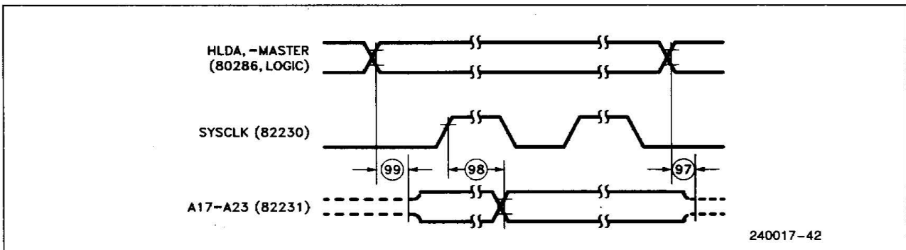
Figure 28. 82231 A17 to A23 Timing
