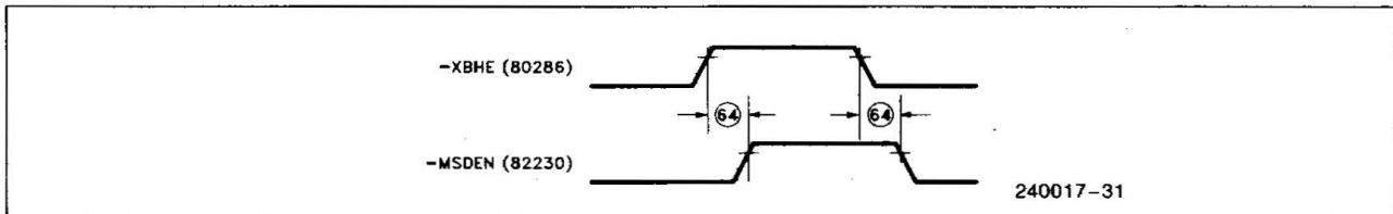
Figure 17. 82230 XHBE Timing
