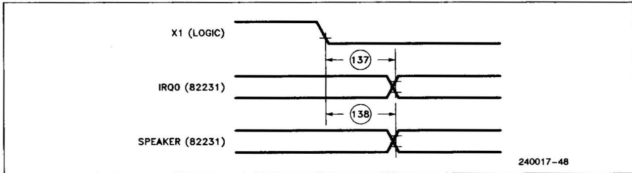
Figure 34. 82231 IRQ0 and SPEAKER Timing
