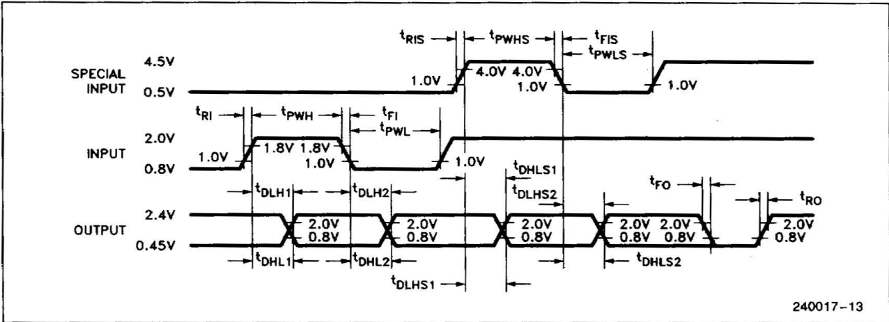
Figure 1A. Delay Time and Pulse Width Measurements
