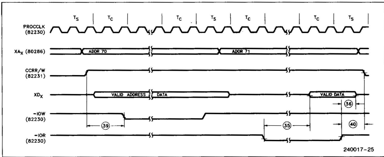
Figure 11. 82230 6818 Read Cycle
