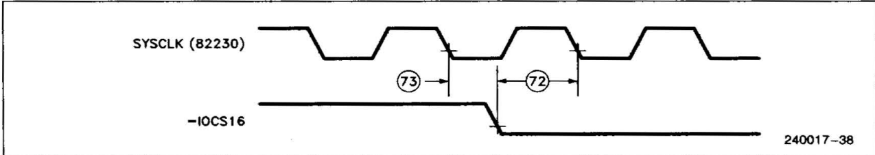
Figure 24. Bus Control Signal Timing
