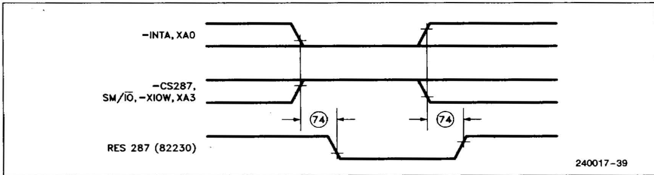
Figure 25. RES 287 Timing
