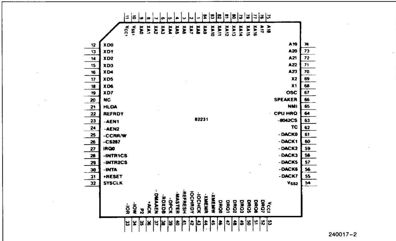
Pin Diagram 82231
