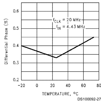
Differential Phase vs Temperature
