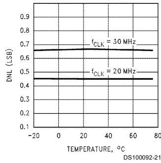
DNL vs Temp at f_{CLK}
