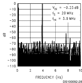
Spectral Response at f_{CLK} = 20 MSPS
