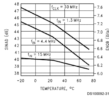
SINAD/ENOB vs Temp
