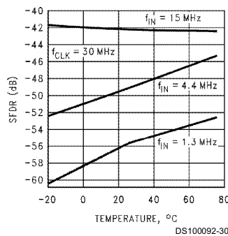
SFDR vs Temp and f_{IN}
