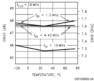
SINAD/ENOB vs Temp
