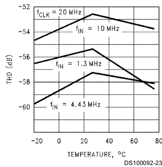
THD vs Temp
