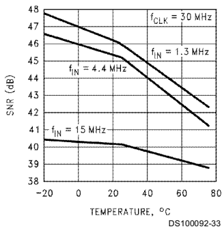
SNR vs Temp at f_{CLK}
