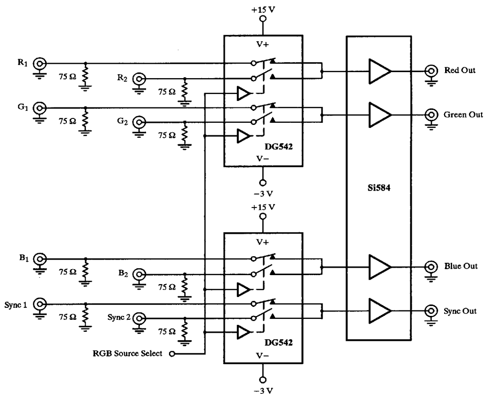
Figure 9. RGB Selector Using Two DG542s
