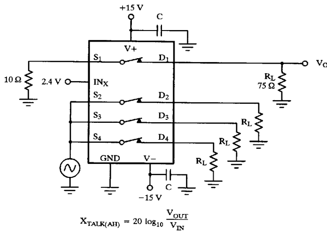
Figure 6. All Hostile Crosstalk
