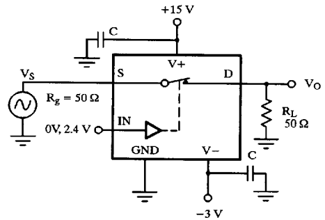
Figure 5. Bandwidth
