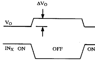
\Delta V_O = measured voltage error due to charge injection The charge injection in coulombs is \Delta Q = C_L \times \Delta V_O
