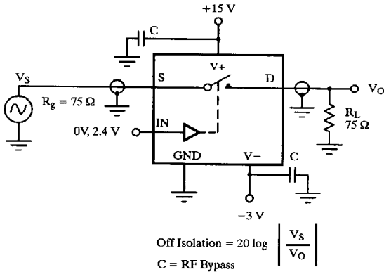
Figure 4. Off Isolation
