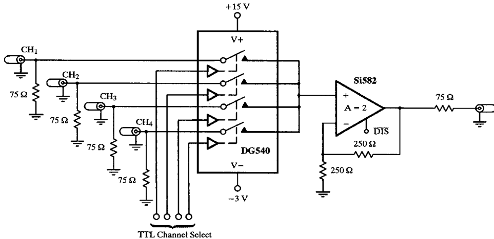
Figure 8. 4 by 1 Video Multiplexing Using the DG540
