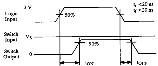
Figure 2. Switching Time
