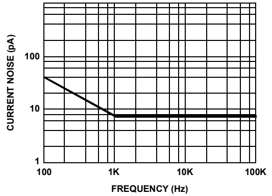
FIGURE 20. CURRENT NOISE
