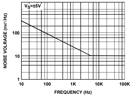
FIGURE 10. EQUIVALENT INPUT VOLTAGE NOISE vs FREQUENCY
