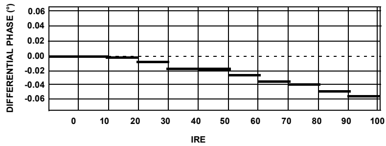
FIGURE 28. DIFFERENTIAL PHASE (°)
