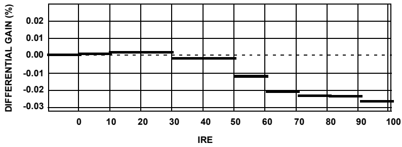
FIGURE 27. DIFFERENTIAL GAIN (%)
