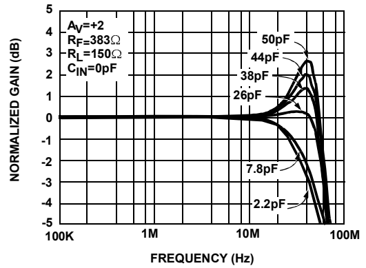
FIGURE 24. GAIN vs FREQUENCY FOR VARIOUS C_L
