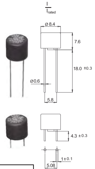
Dimensions [mm]
