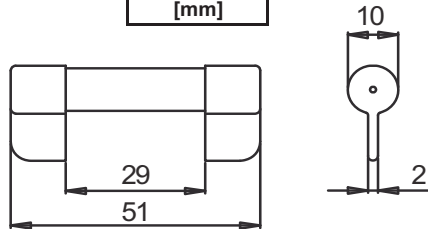
Dimensions [mm]
