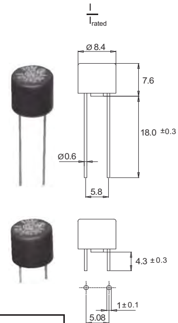
Dimensions [mm]
