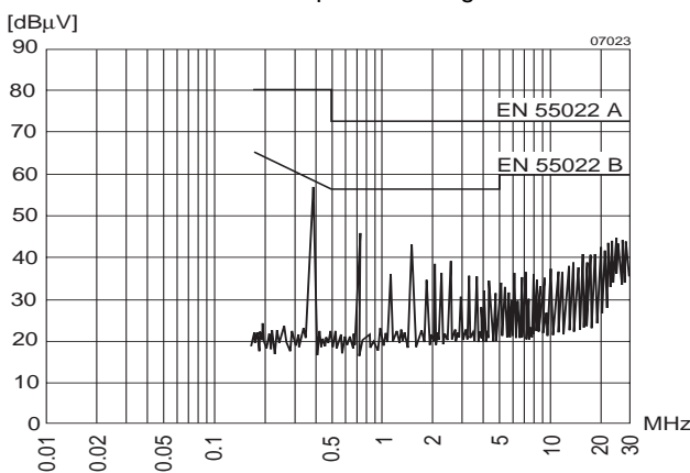
Fig. 15 Typical disturbance voltage (quasi-peak) at the input according to CISPR 11/EN 55011 and CISPR 22/EN 55022 measured at V_{i,nom} and I_{o,nom} . Output leads 0.1 m, twisted. (40IMX7-15-15). External capacitor (1 μF ceramic or film) required at the input for 70IMX7, 110IMX7 types.
