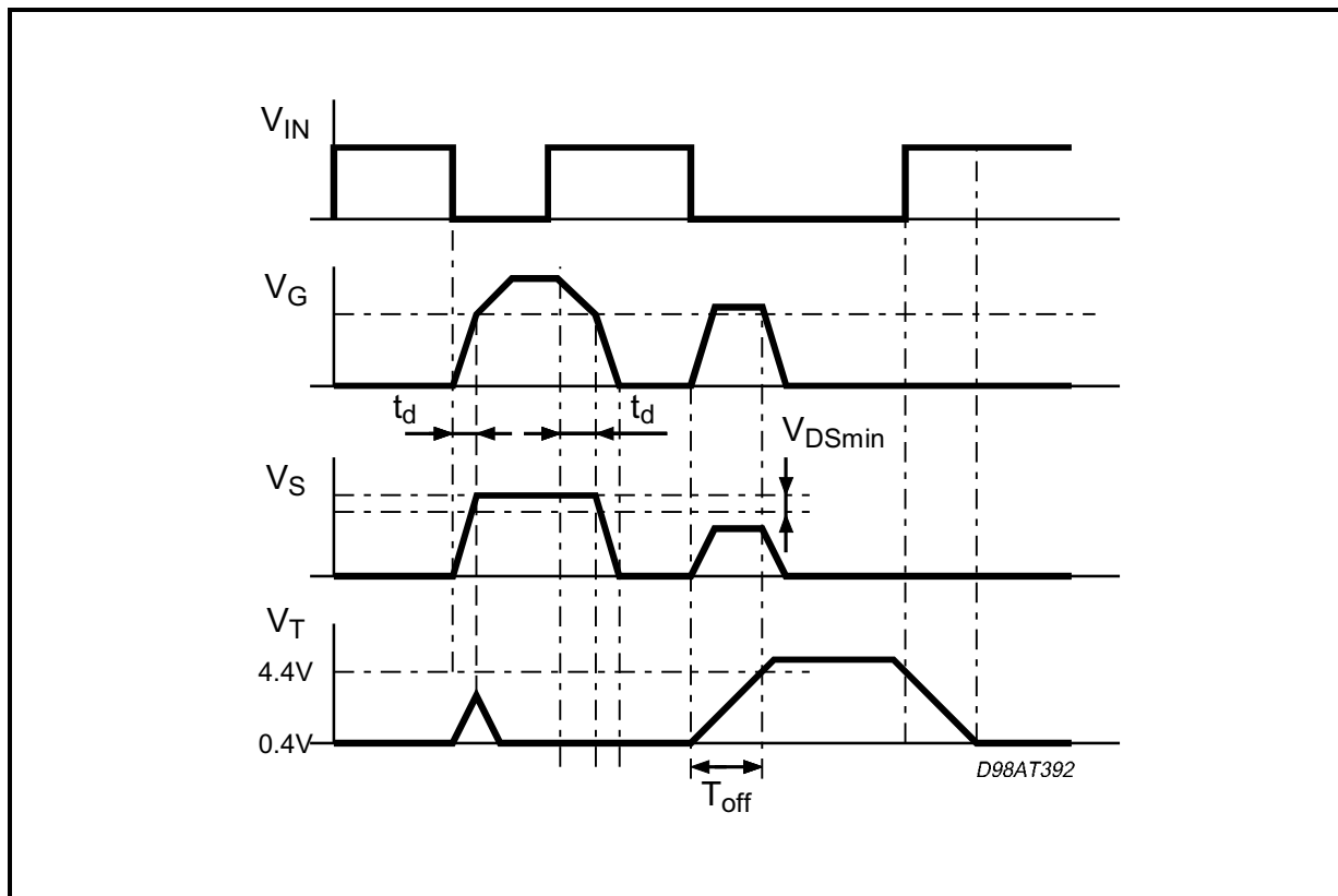
Figure 4. Timing Characteristic.
