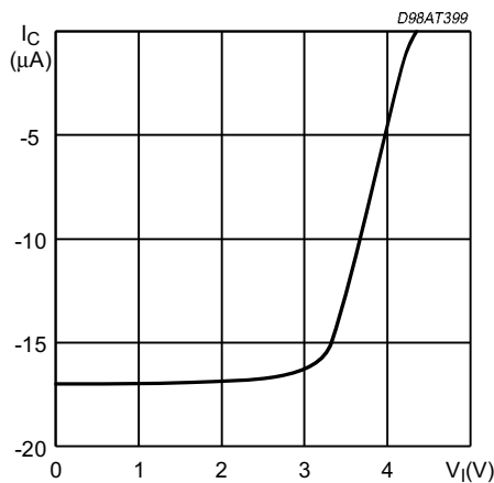
Figure 11. Input Current as function of the Input Voltage
