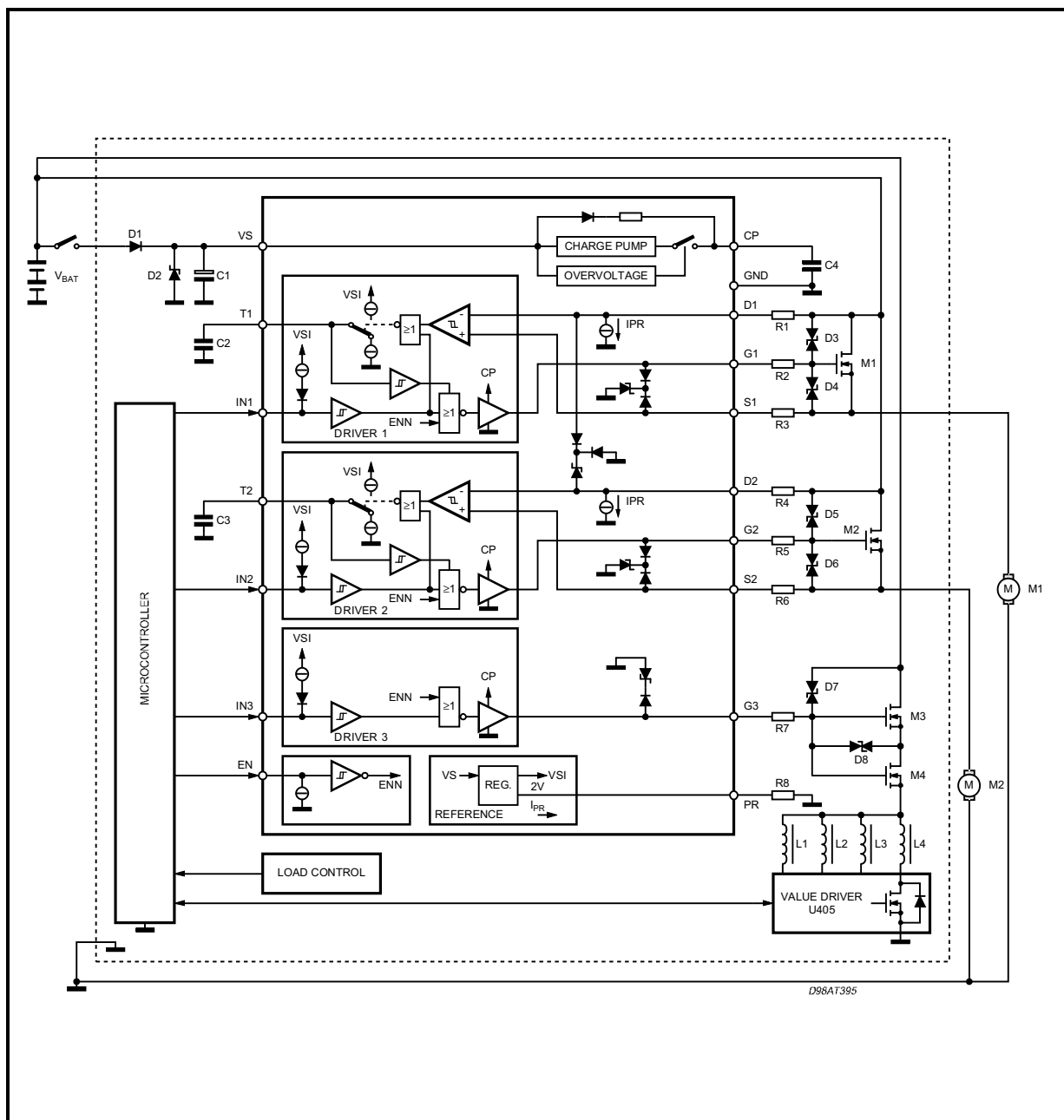
Figure 7. Application Circuit.
