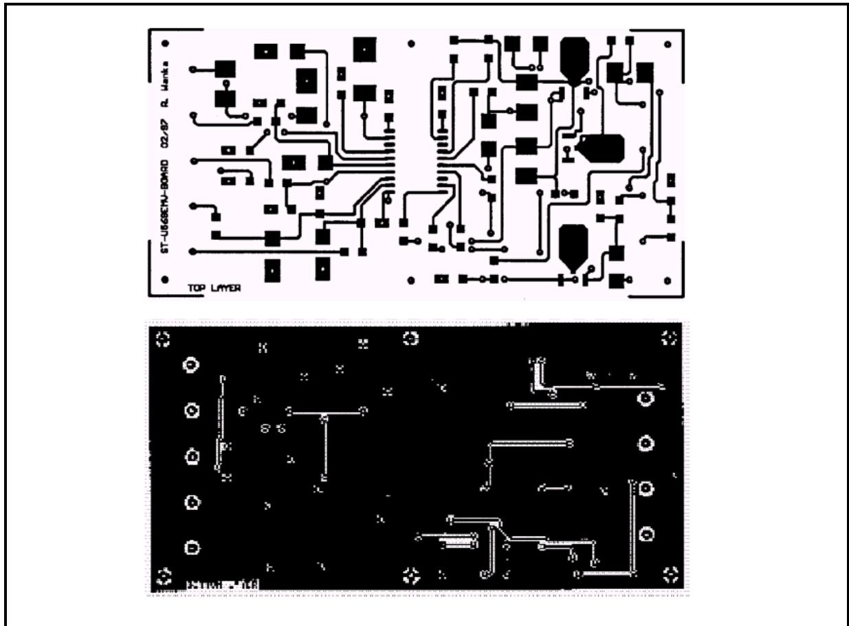
Figure 14: PCB Board
