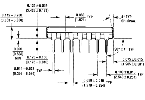
Moulded Dual-In-Line Package (N) Order Number LM319AN or LM319N NS Package Number N14A
