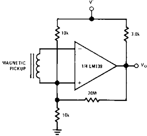
Transducer Amplifier
