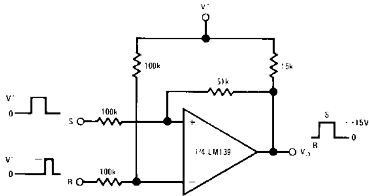
Bi-Stable Multivibrator
