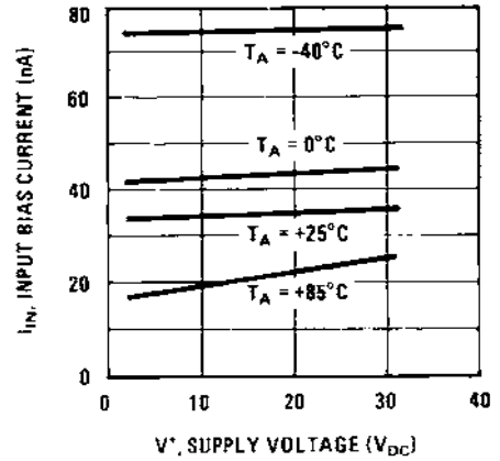
Input Current
