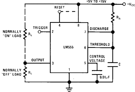
FIGURE 1. Monostable
