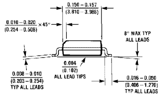
Small Outline Package (M) Order Number LM555CM NS Package Number M08A
