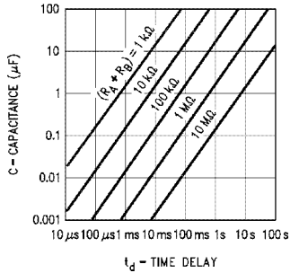
FIGURE 3. Time Delay
