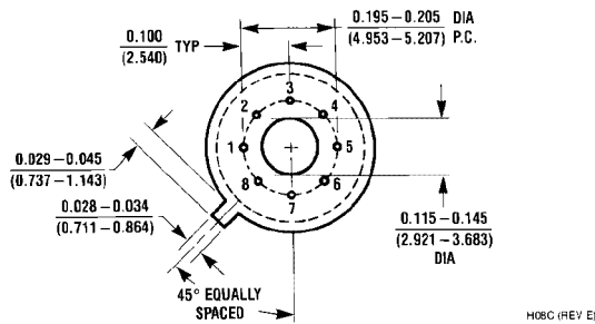
Metal Can Package (H) Order Number LM555H or LM555CH NS Package Number H08C
