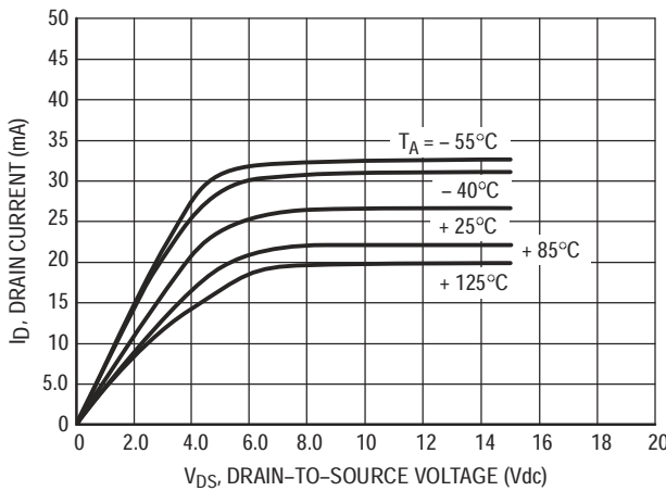
Figure 6. V_{GS} = 15 Vdc
