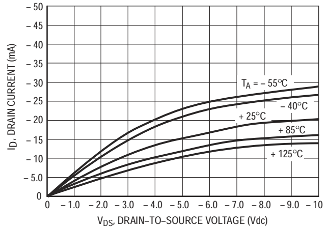
Figure 5. V_{GS} = -10 Vdc
