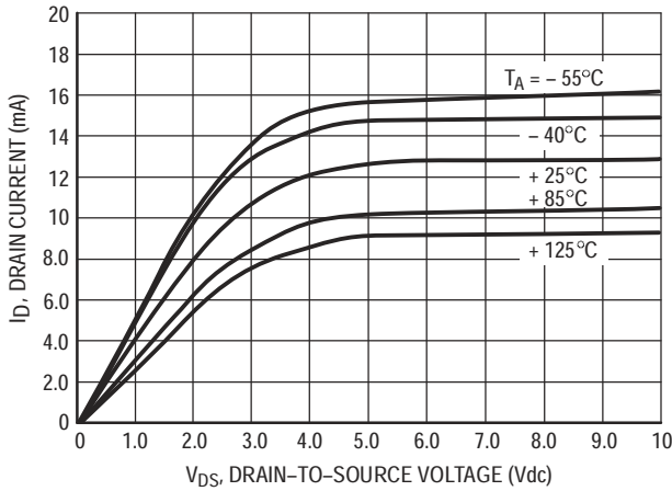
Figure 4. V_{GS} = 10 Vdc
