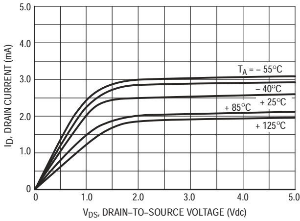
Figure 2. V_{GS} = 5.0 Vdc
