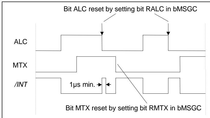
Figure 11-1: Multiple-interrupt events
