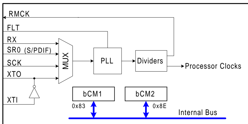
Figure 9-1: Clock Manager
