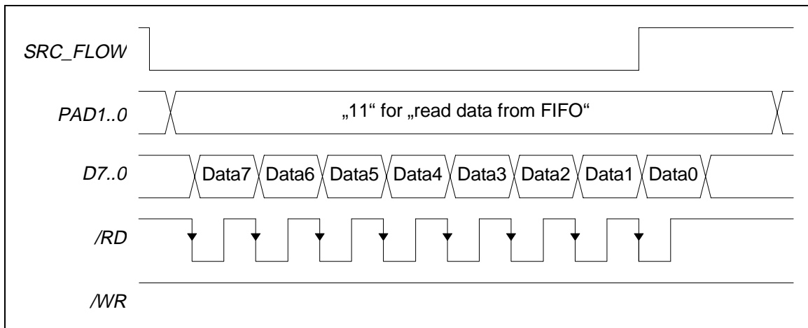
Figure 8-13 Reading 8 bytes Timing (SP in Parallel-Async. mode)
