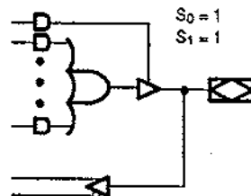
Figure 3d. Combinatorial/Active High
