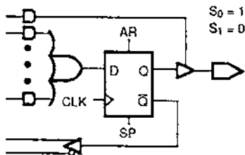
Figure 3b. Registered/Active High
