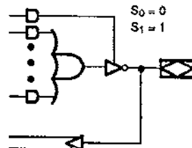
Figure 3c. Combinatorial/Active Low
