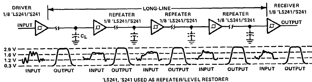
'LS241, 'S241 USED AS REPEATER/LEVEL RESTORER
