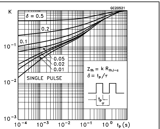
Figure 6. Thermal impedance for TO-247
