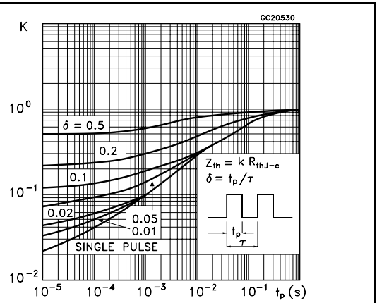
Figure 4. Thermal impedance for TO-220FP
