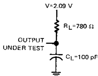
FIGURE 1 – TYPICAL OUTPUT LOAD CIRCUIT
