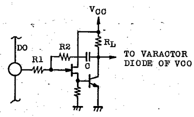
Example of active low pass filter
