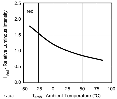
Figure 26. Relative Luminous Intensity vs. Ambient Temperature
