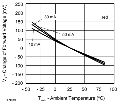
Figure 25. Change of Forward Voltage vs. Ambient Temperature
