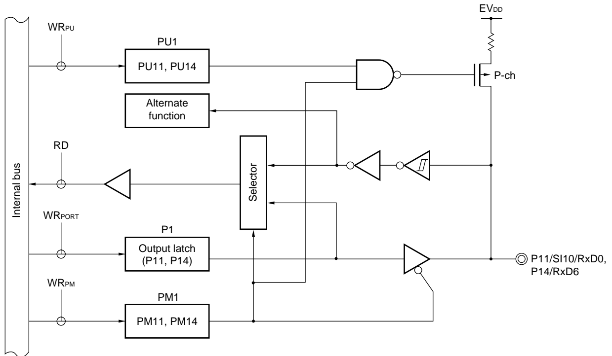
Figure 5-8. Block Diagram of P11 and P14
