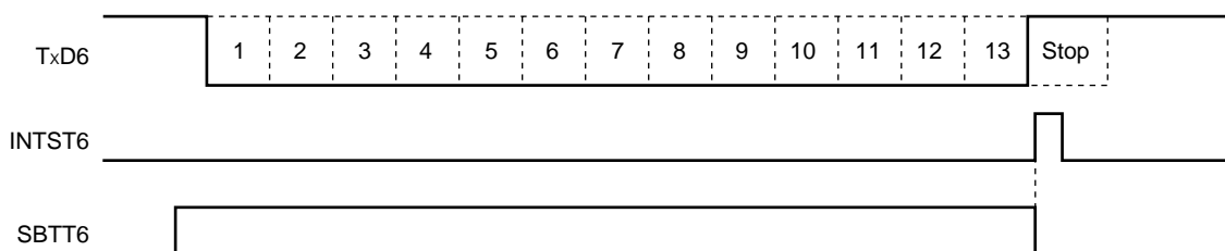
Figure 15-22. SBF Transmission
