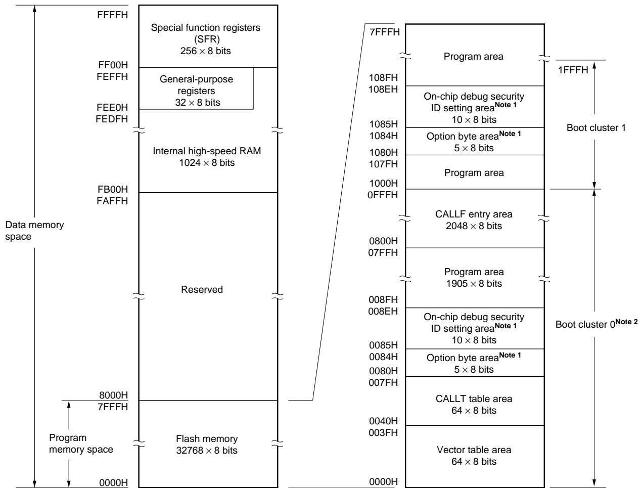
Figure 3-5. Memory Map ( \mu PD78F0503D, 78F0503DA, 78F0513D, and 78F0513DA)
