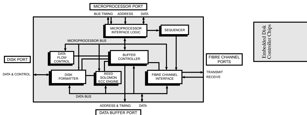
Figure 1. FTEC440 Block Diagram
