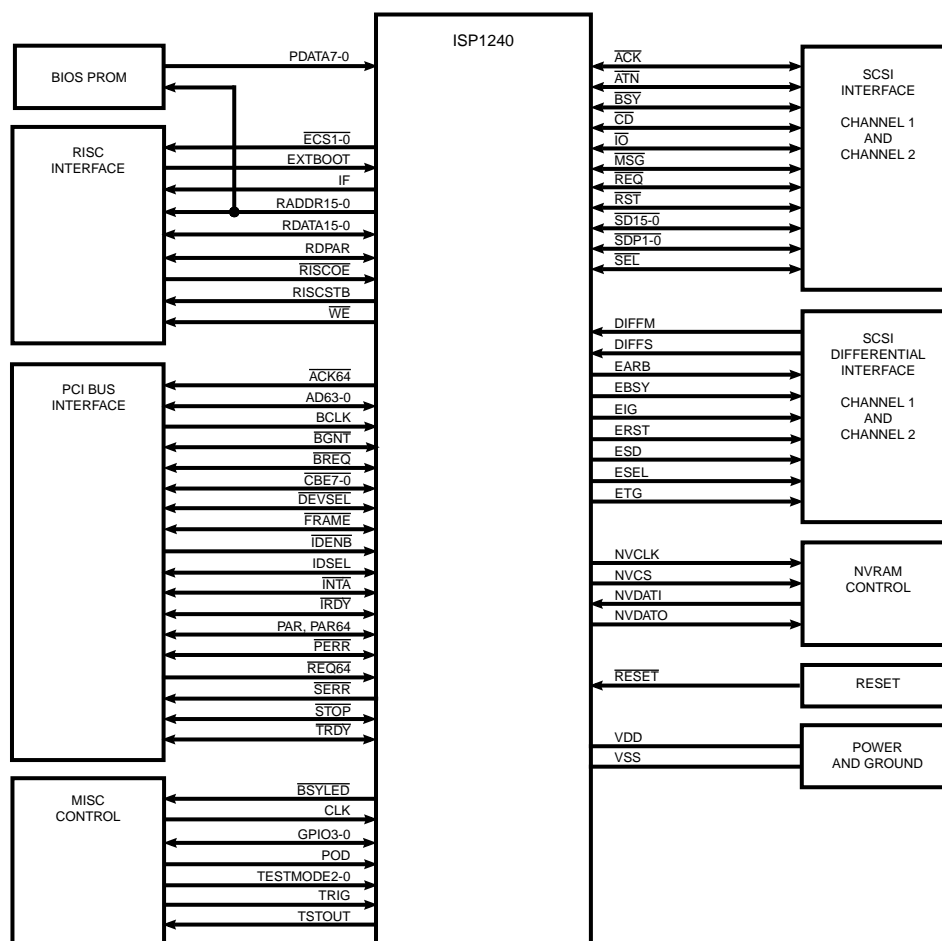
Figure 3. ISP1240 Functional Signal Grouping
