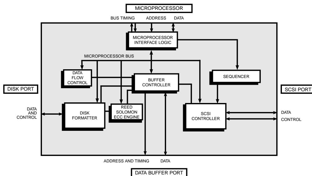
Figure 1. TEC420 Block Diagram
