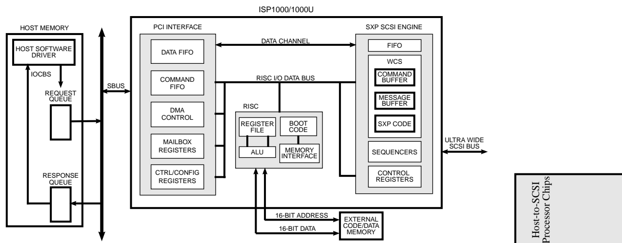
Figure 1. ISP1000/1000U Block Diagram
