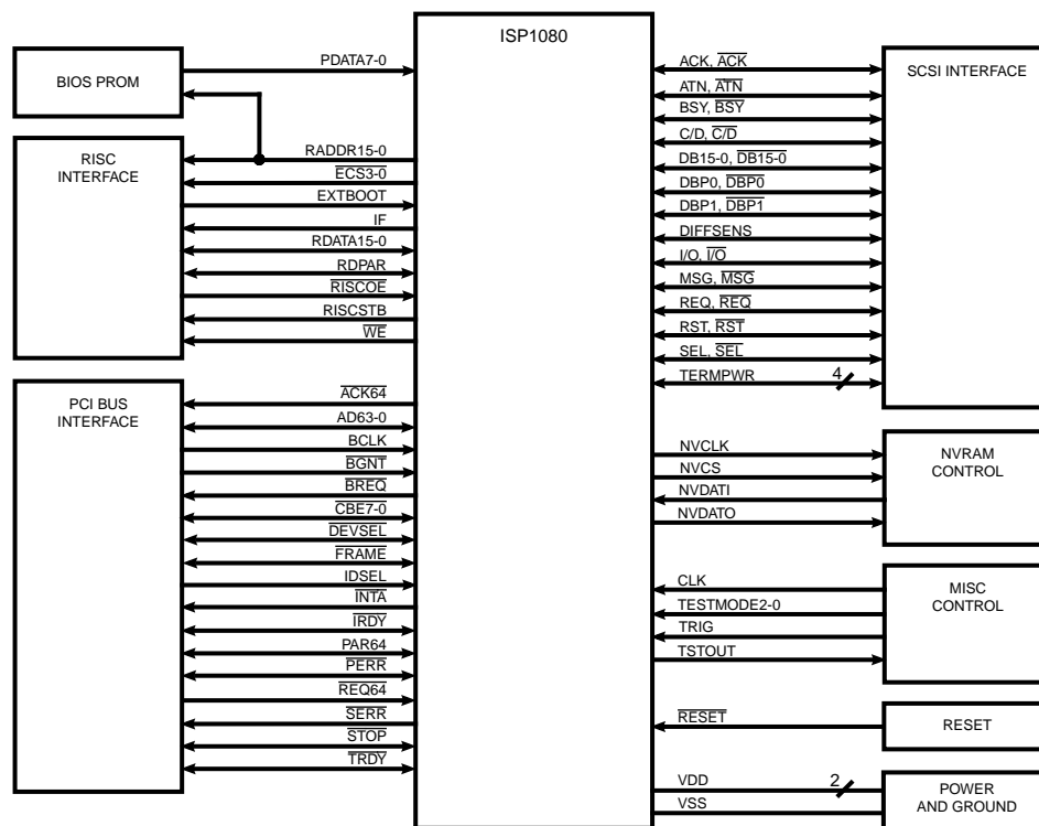
Figure 3. ISP1080 Functional Signal Grouping
