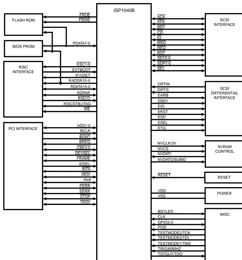
Figure 3. ISP1040B Functional Signal Grouping
