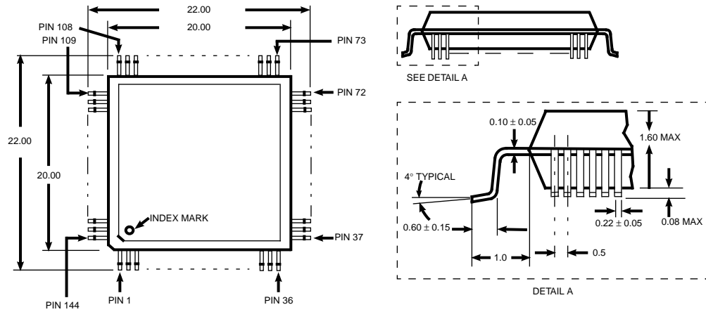
Figure 9. TEC336 144-Pin PQFP Mechanical Drawings
