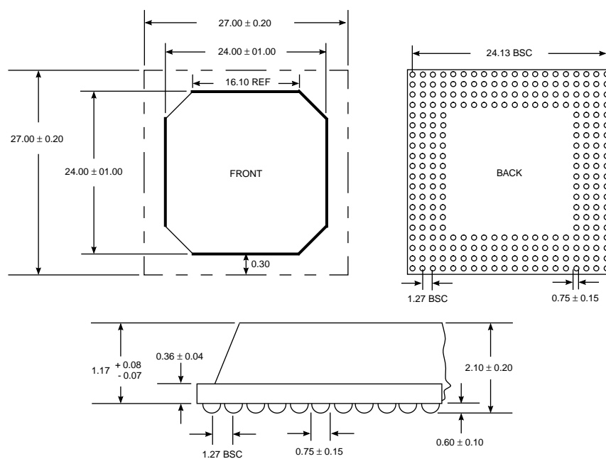
Figure 4. ISP2100 Mechanical Drawings
