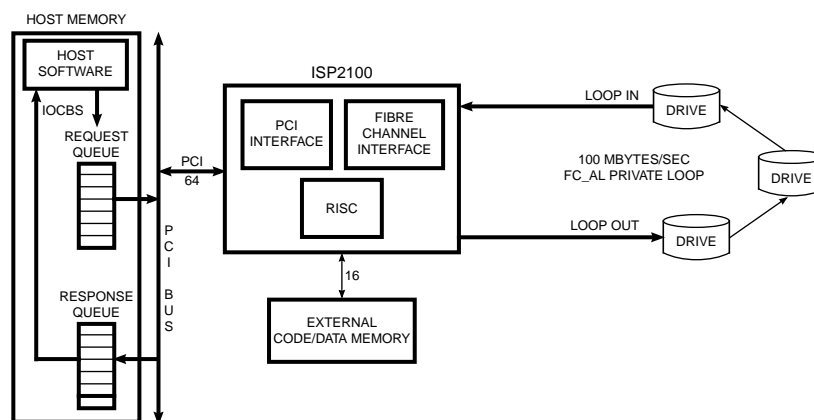
Figure 2. I/O Subsystem Design Using the ISP2100
