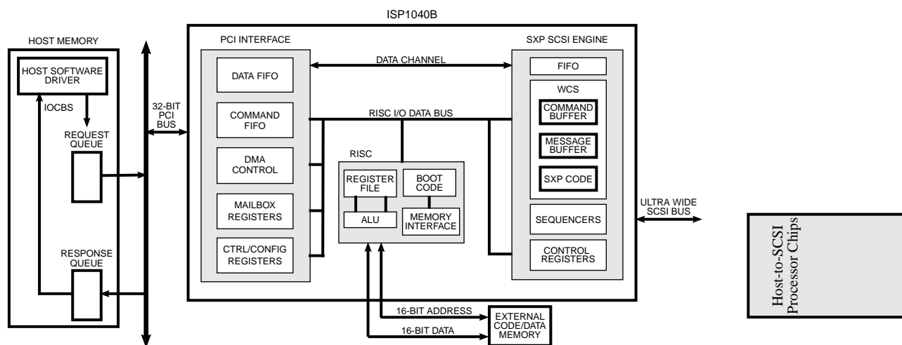
Figure 1. ISP1040B Block Diagram
