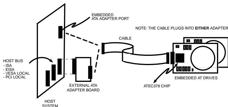
Figure 2. ATEC378 Chip Within a Host System
