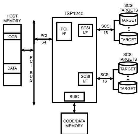
Figure 2. I/O Subsystem Design Using the ISP1240
