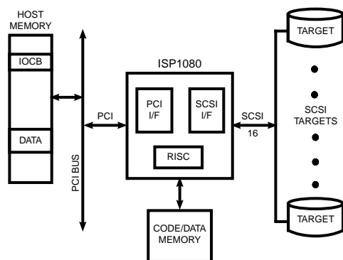
Figure 2. I/O Subsystem Design Using the ISP1080
