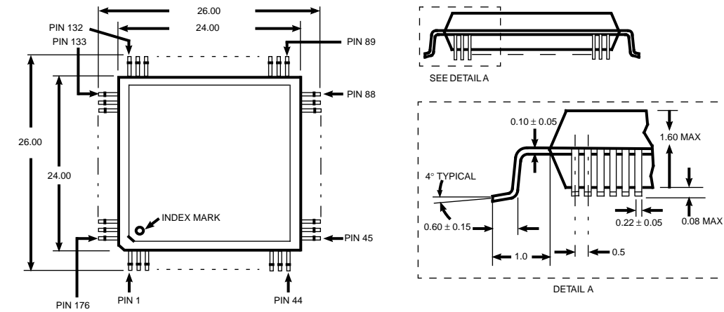
Figure 10. TEC356 176-Pin PQFP Mechanical Drawings
