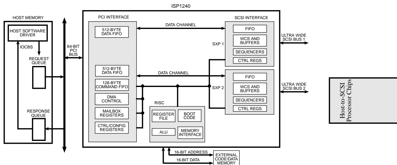
Figure 1. ISP1240 Block Diagram
