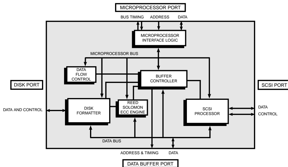
Figure 1. TEC376/386 Block Diagram
