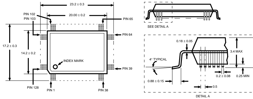
Figure 13. TEC420 128-Pin PQFP Mechanical Drawings
