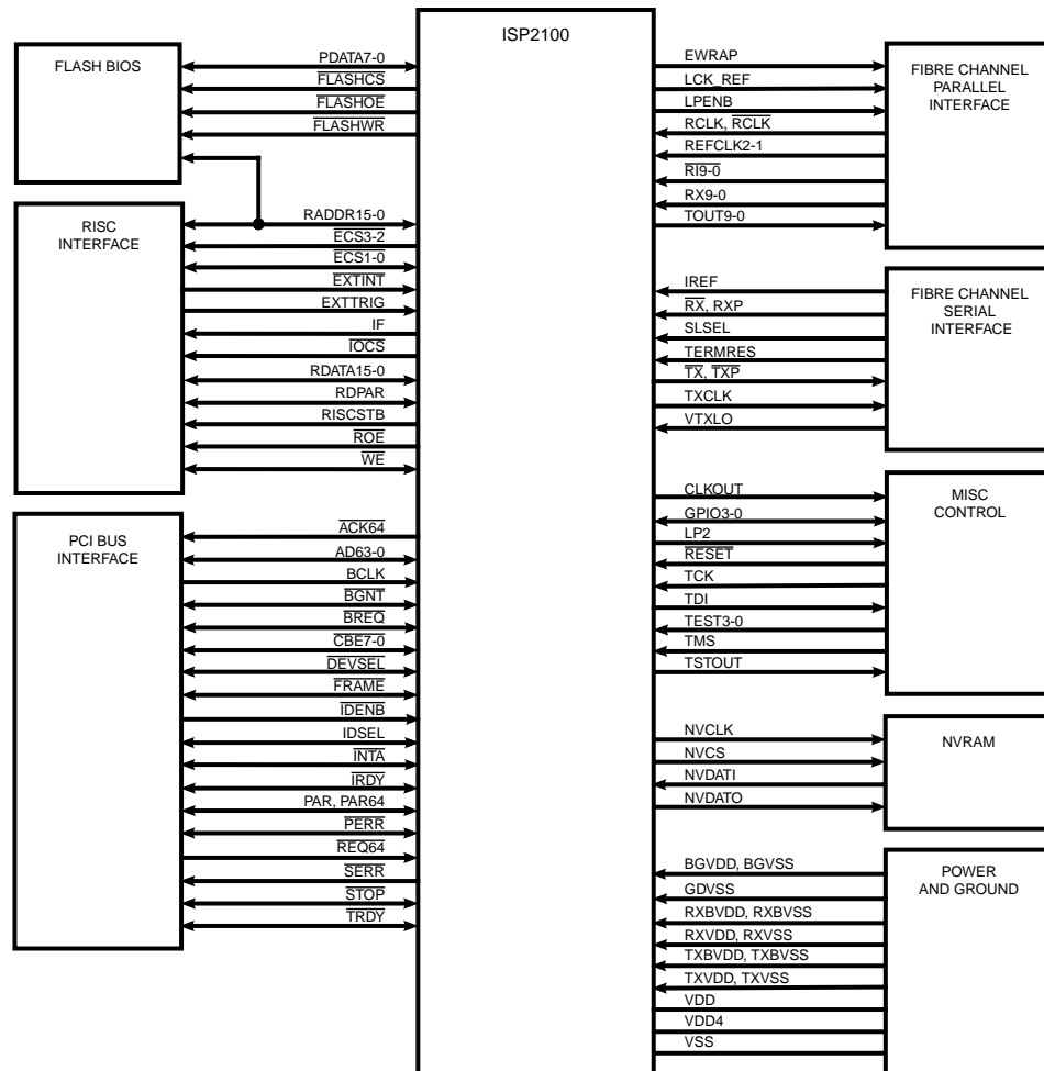
Figure 3. ISP2100 Functional Signal Grouping
