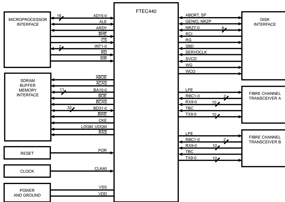
Figure 2. FTEC440 Functional Signal Grouping
