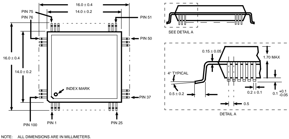
Figure 11. TEC376 100-Pin PQFP Mechanical Drawings
