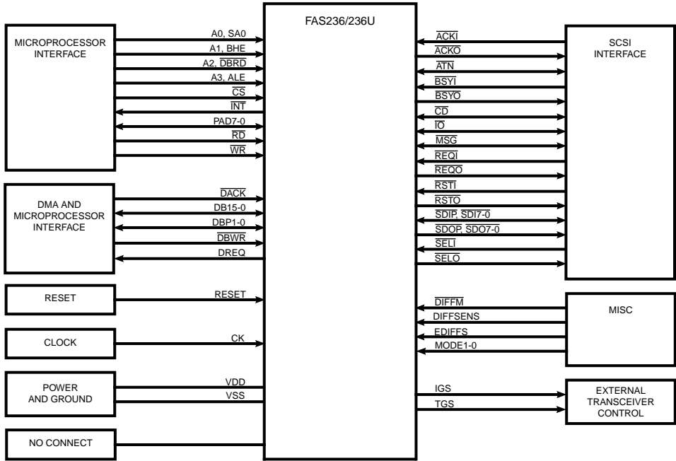
Figure 3. FAS236/236U Functional Signal Grouping
