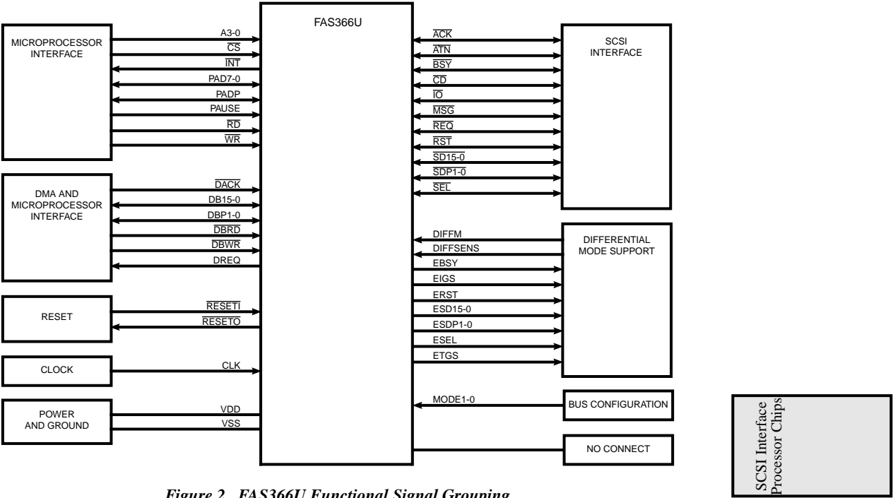
Figure 2. FAS366U Functional Signal Grouping
