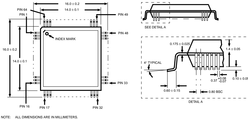
Figure 3. FAS209 64-Pin TQFP Mechanical Drawings
