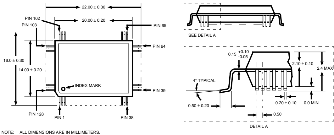
Figure 1. ATEC378 128-Pin PQFP Mechanical Drawings
