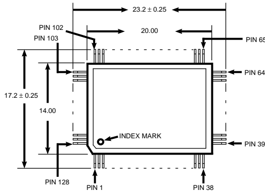
Figure 6. FAS366/366U 128-Pin PQFP Mechanical Drawings
