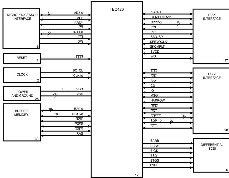
Figure 2. TEC420 Functional Signal Grouping
