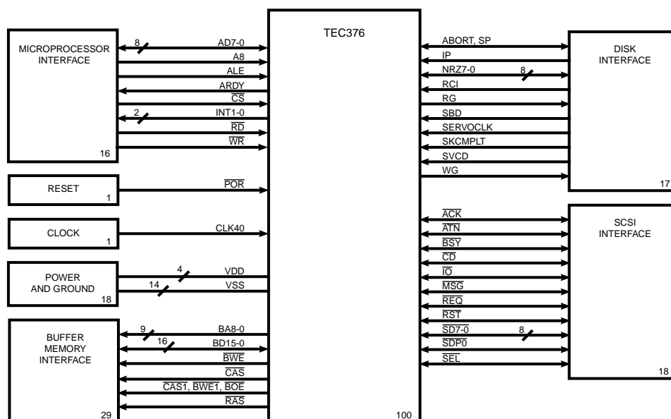
Figure 2. TEC376 Functional Signal Grouping
