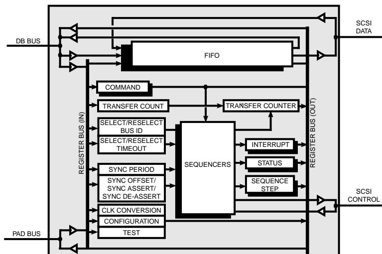
Figure 1. FAS209 Block Diagram
