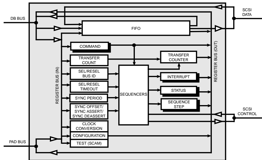
Figure 1. FAS2x6 Block Diagram
