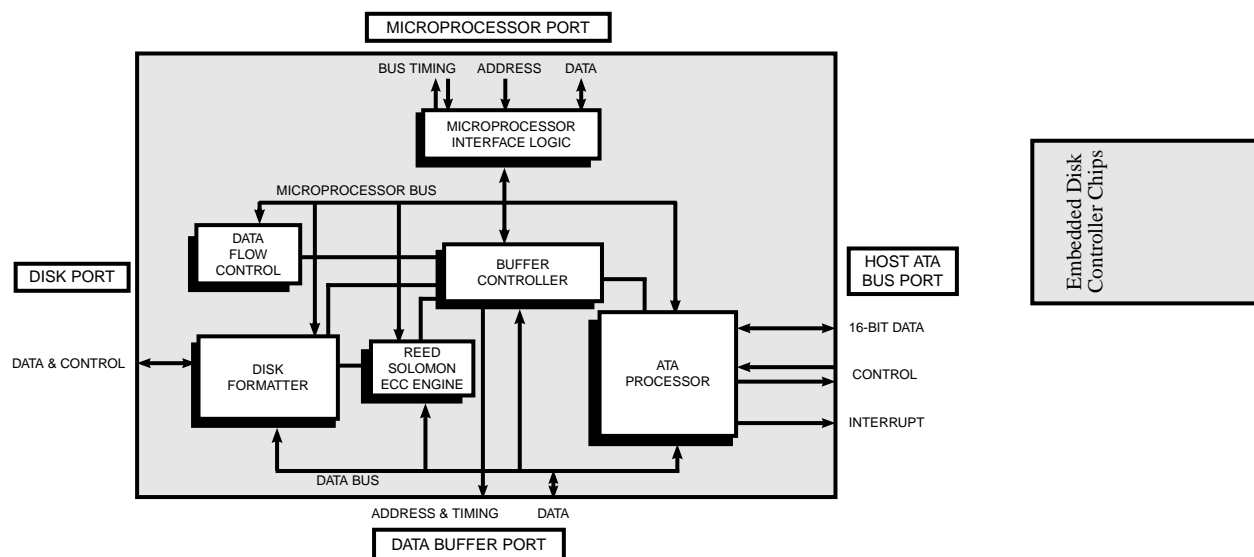
Figure 1. ATEC378 Block Diagram
