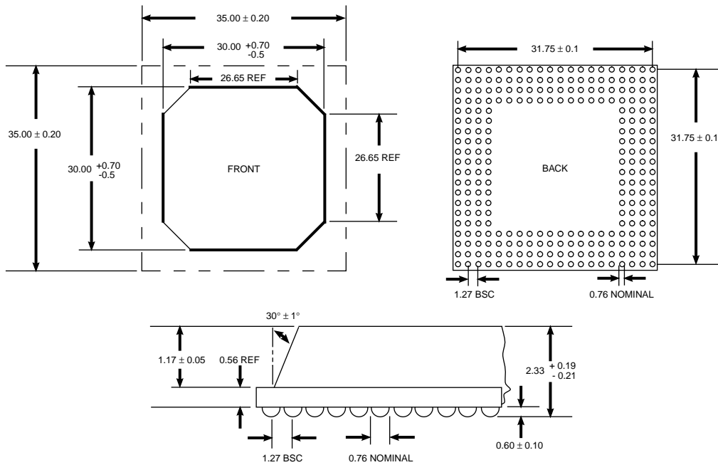
Figure 8. ISP1080/1240 352-Pin BGA Mechanical Drawings
