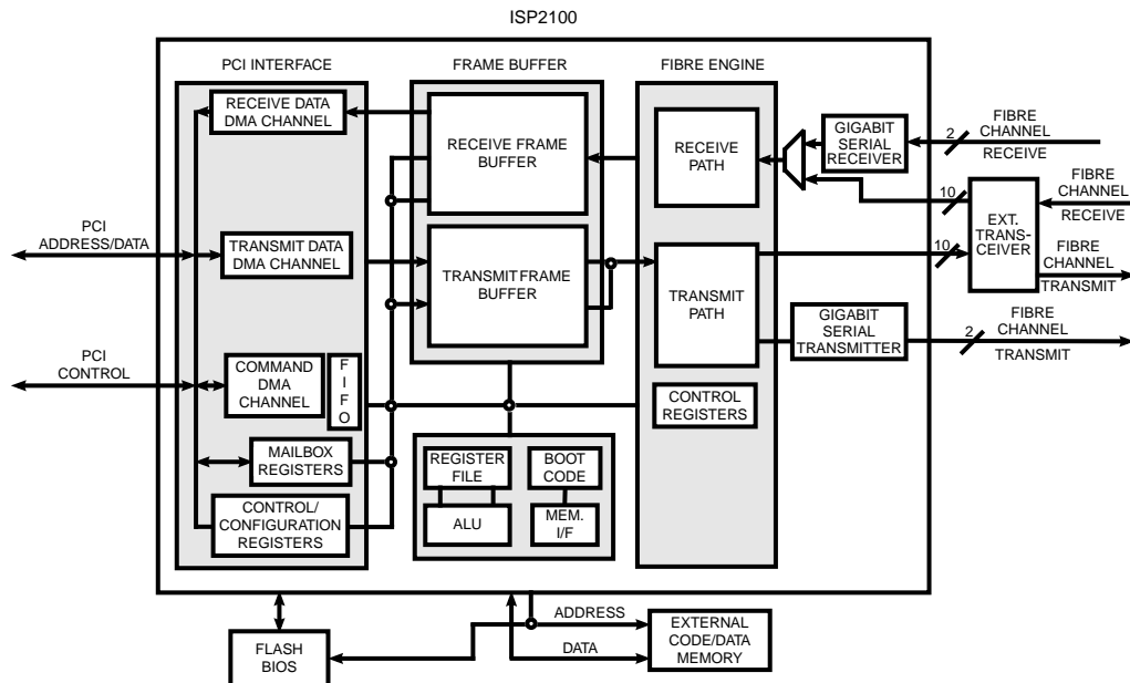
Figure 1. ISP2100 Block Diagram
