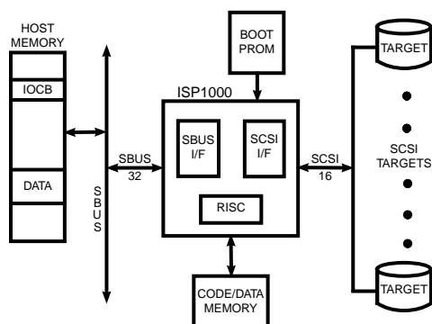
Figure 2. I/O Subsystem Design Using the ISP1000/1000U
