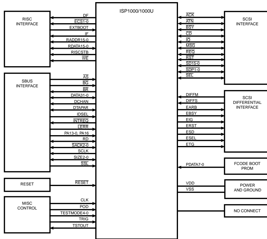
Figure 3. ISP1000/1000U Functional Signal Grouping
