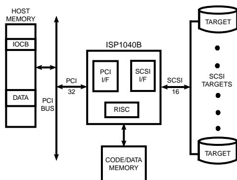
Figure 2. I/O Subsystem Design Using the ISP1040B
