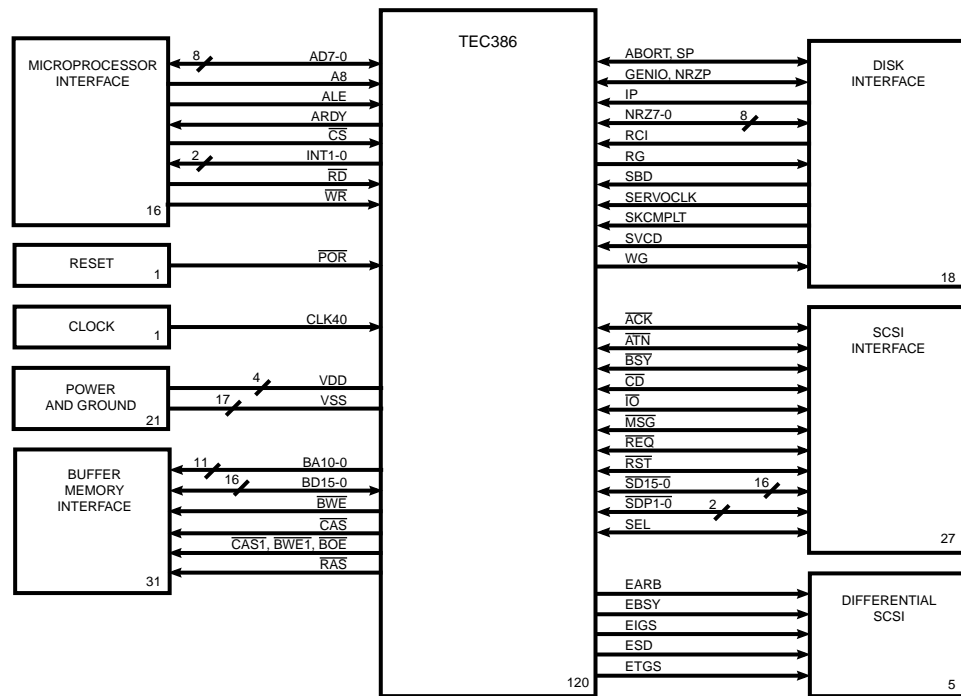
Figure 3. TEC386 Functional Signal Grouping
