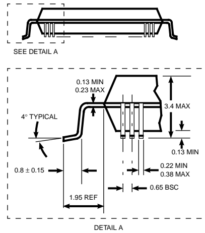
Figure 5. FAS236/236U 100-Pin PQFP Mechanical Drawings
