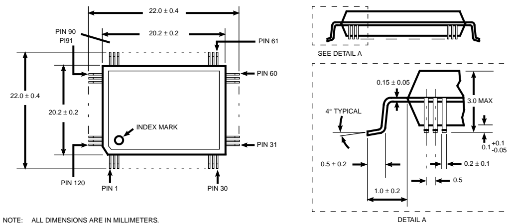
Figure 12. TEC386 120-Pin PQFP Mechanical Drawings
