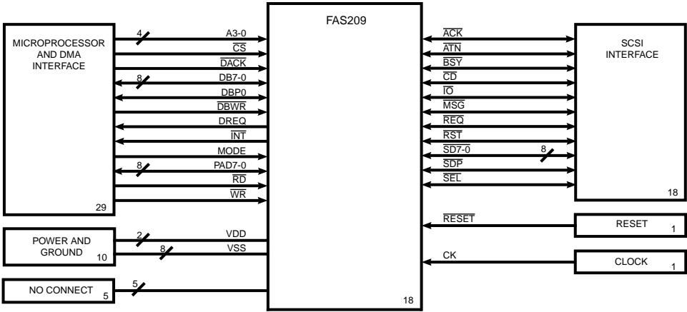
Figure 2. FAS209 Functional Signal Grouping
