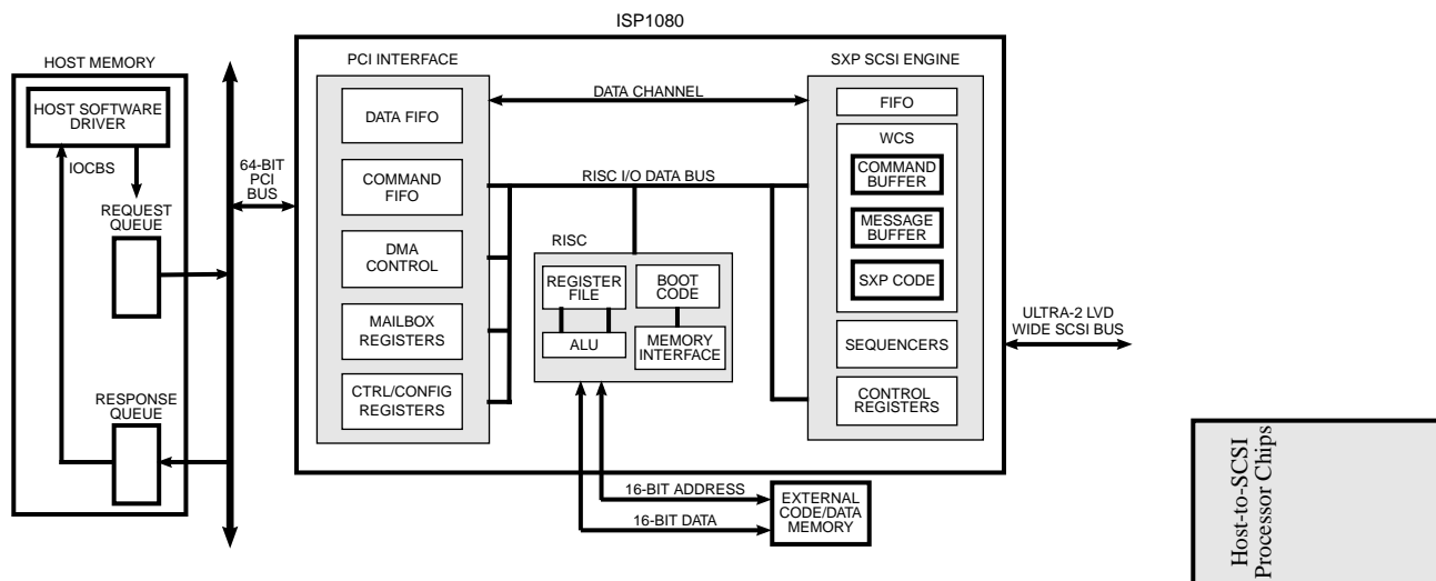
Figure 1. ISP1080 Block Diagram
