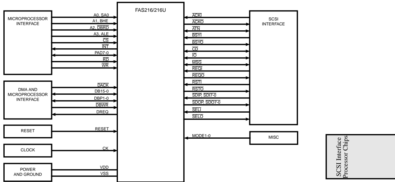
Figure 2. FAS216/216U Functional Signal Grouping
