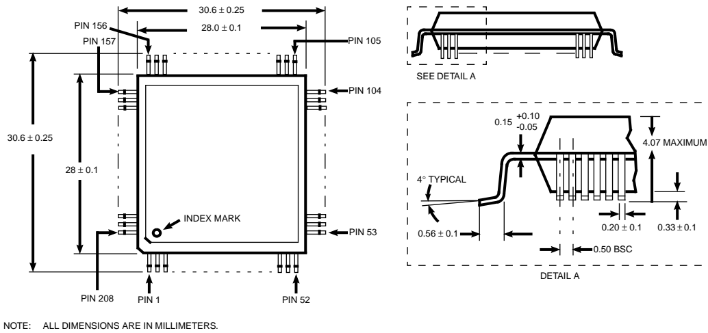
Figure 7. ISP1000/1000U/1040B 208-Pin PQFP Mechanical Drawings
