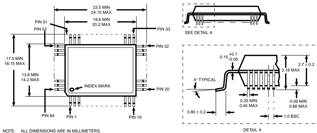
Figure 2. FAS209 64-Pin PQFP Mechanical Drawings
