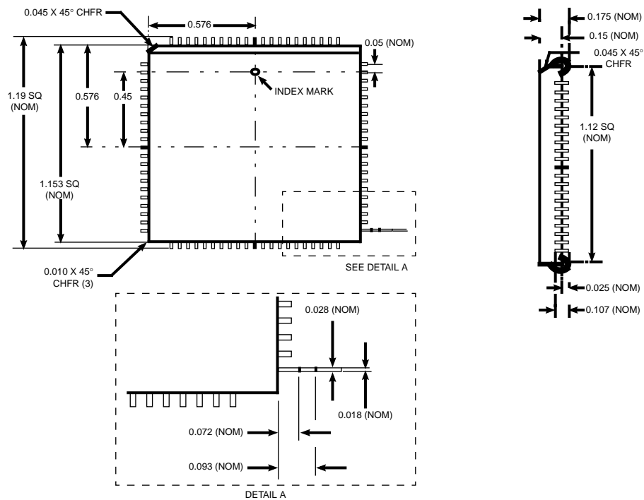
Figure 4. FAS216/216U 84-Pin PLCC Mechanical Drawings
