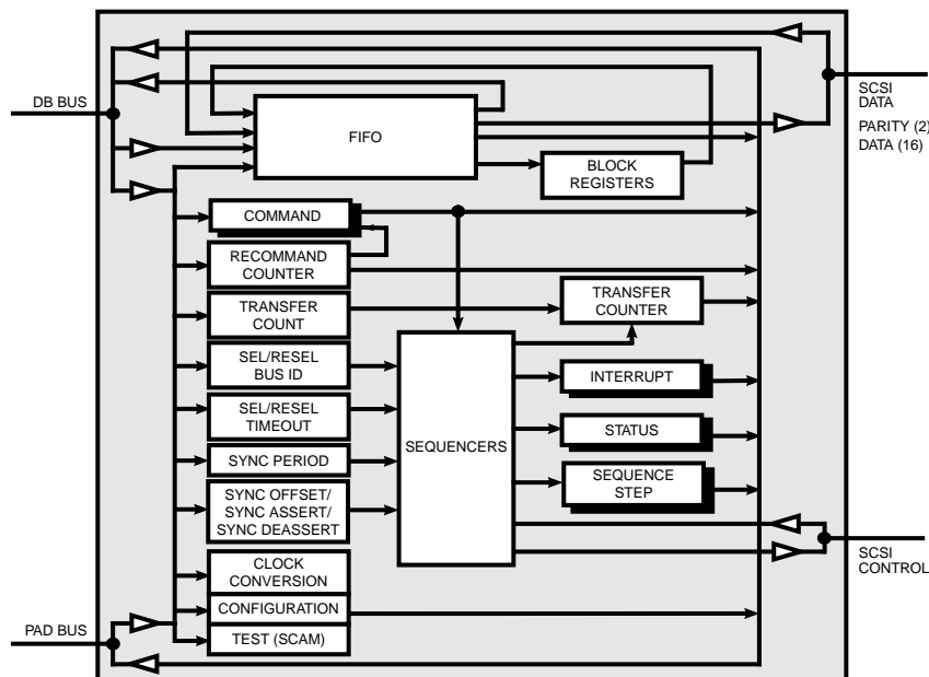
Figure 1. FAS366U Block Diagram
