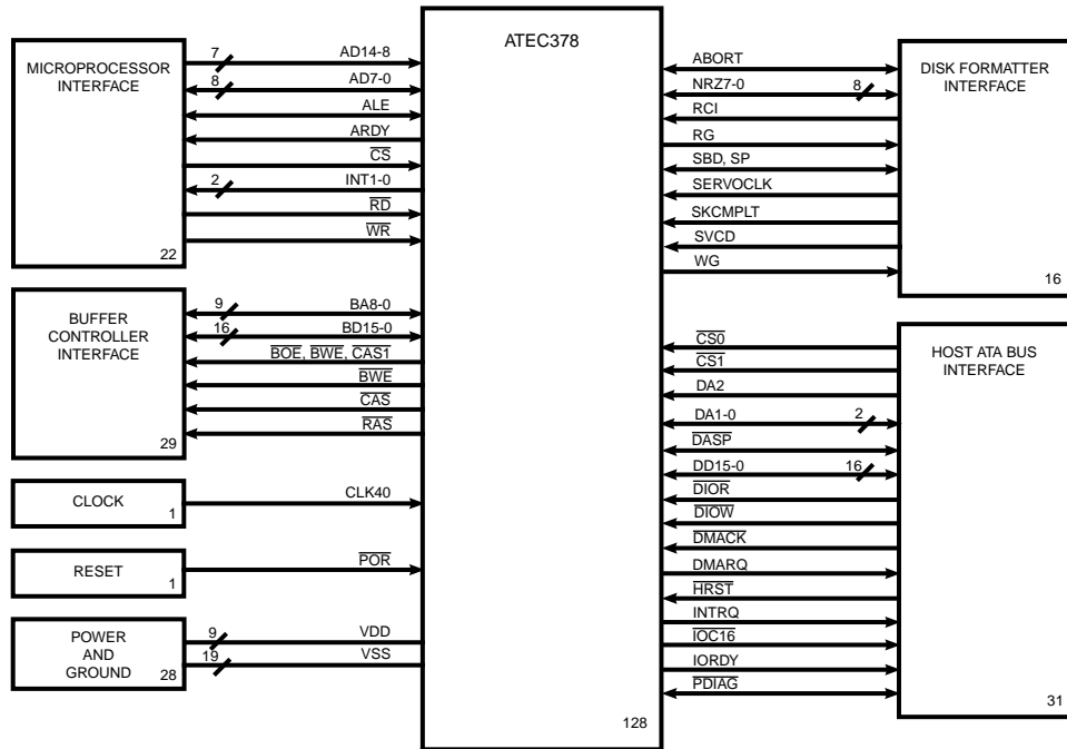
Figure 3. ATEC378 Functional Signal Grouping
