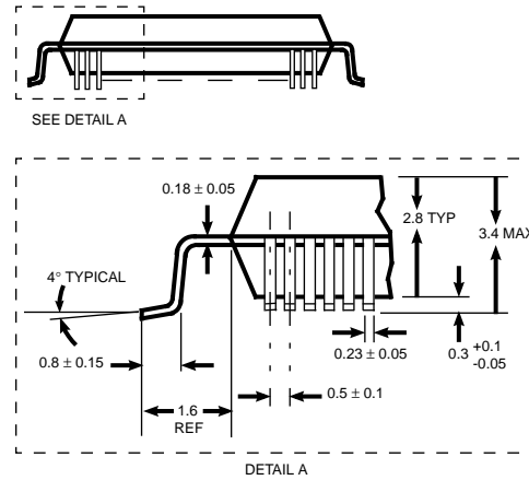
Figure 6. FAS366/366U 128-Pin PQFP Mechanical Drawings
